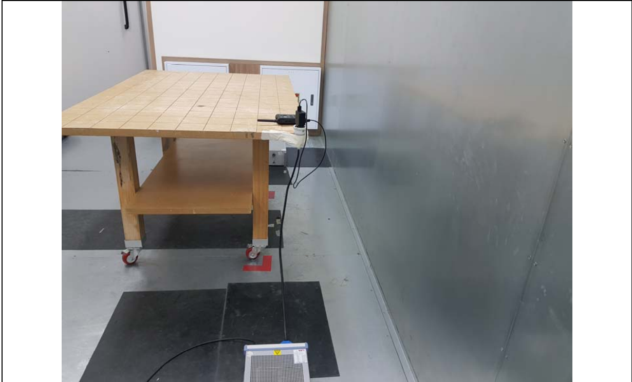
Conducted Emission_REAR_Dipole Antenna
