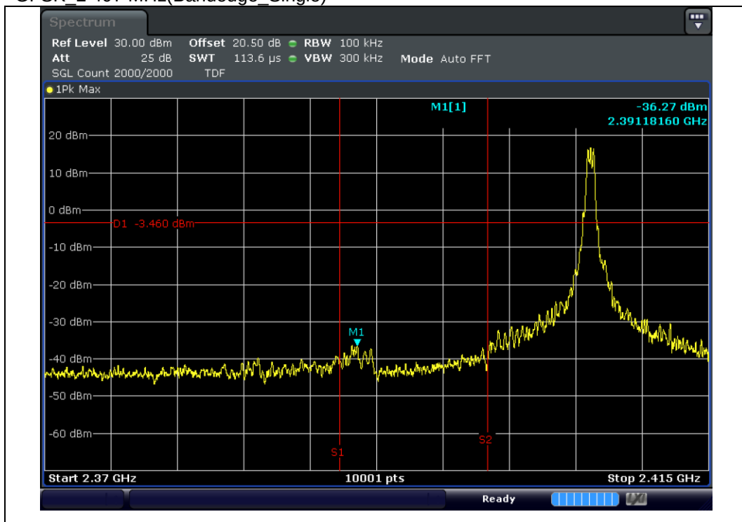
GFSK_2 407 MHz(Bandedge_Single)
