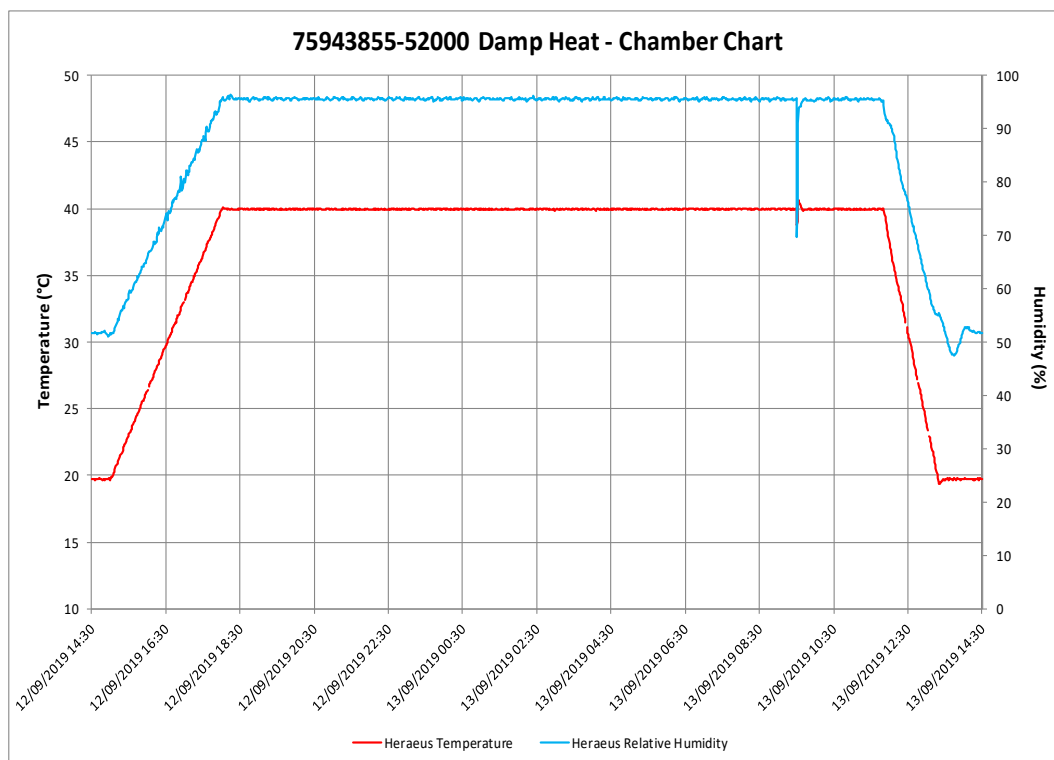
2.2.8.1 – Chamber Chart
