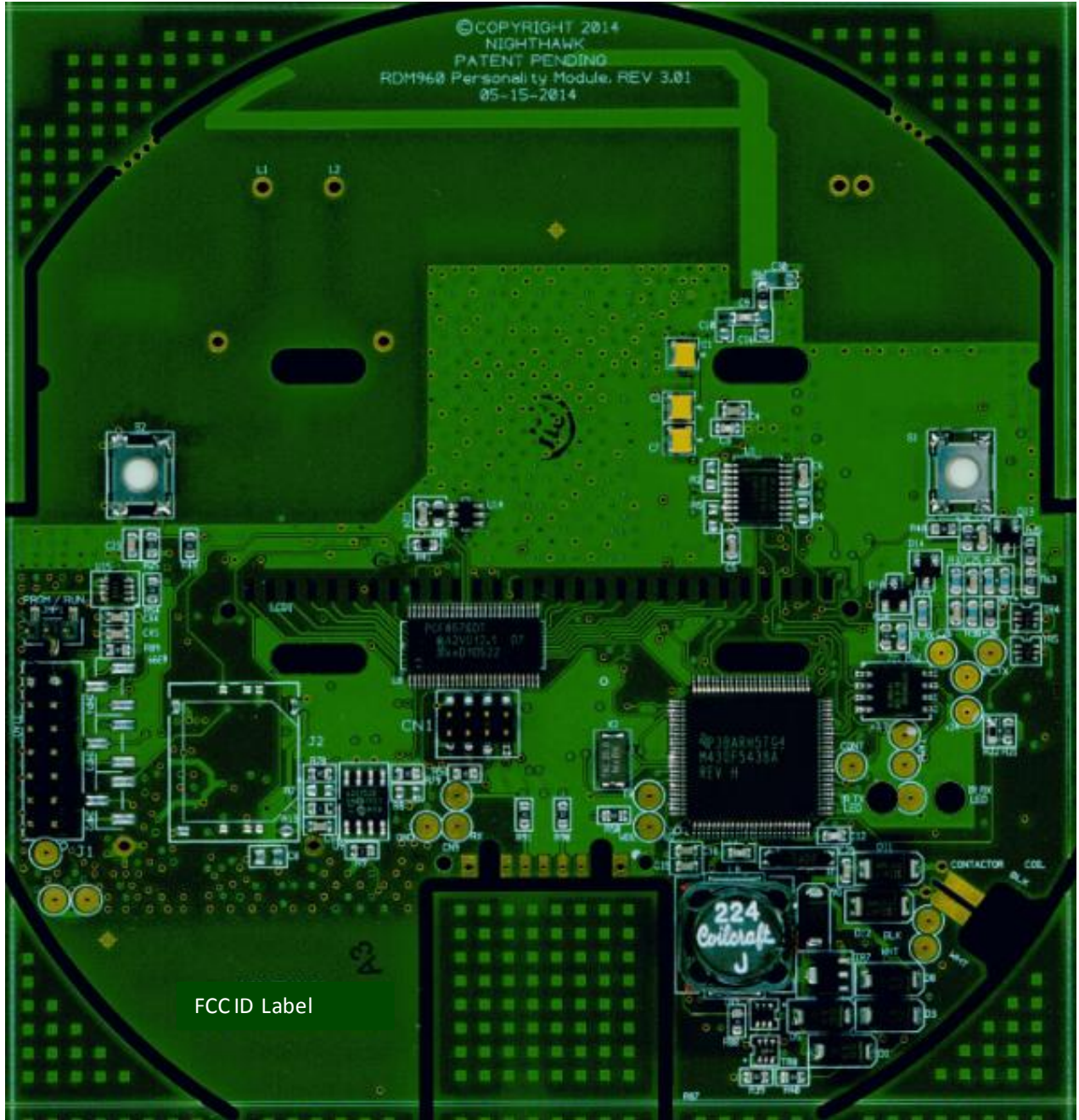
Figure 2. Internal Photos – Bottom Side.
