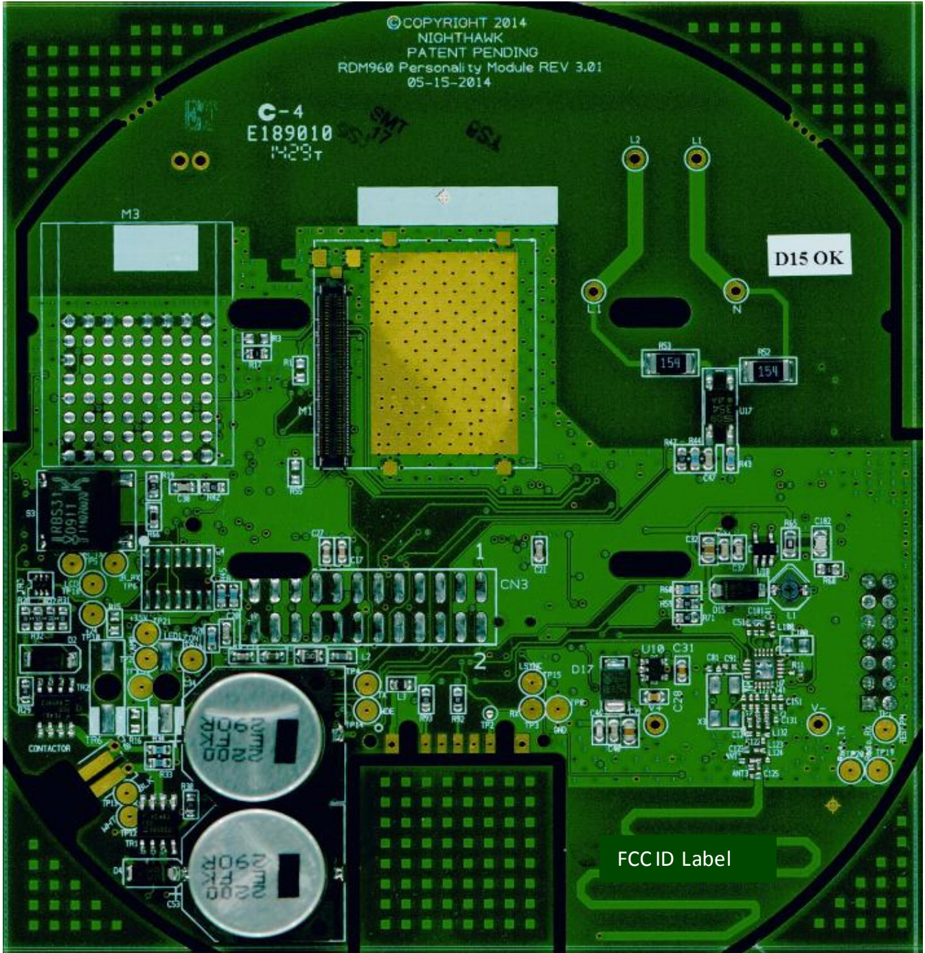
Figure 1. Internal Photos – Top Side.
