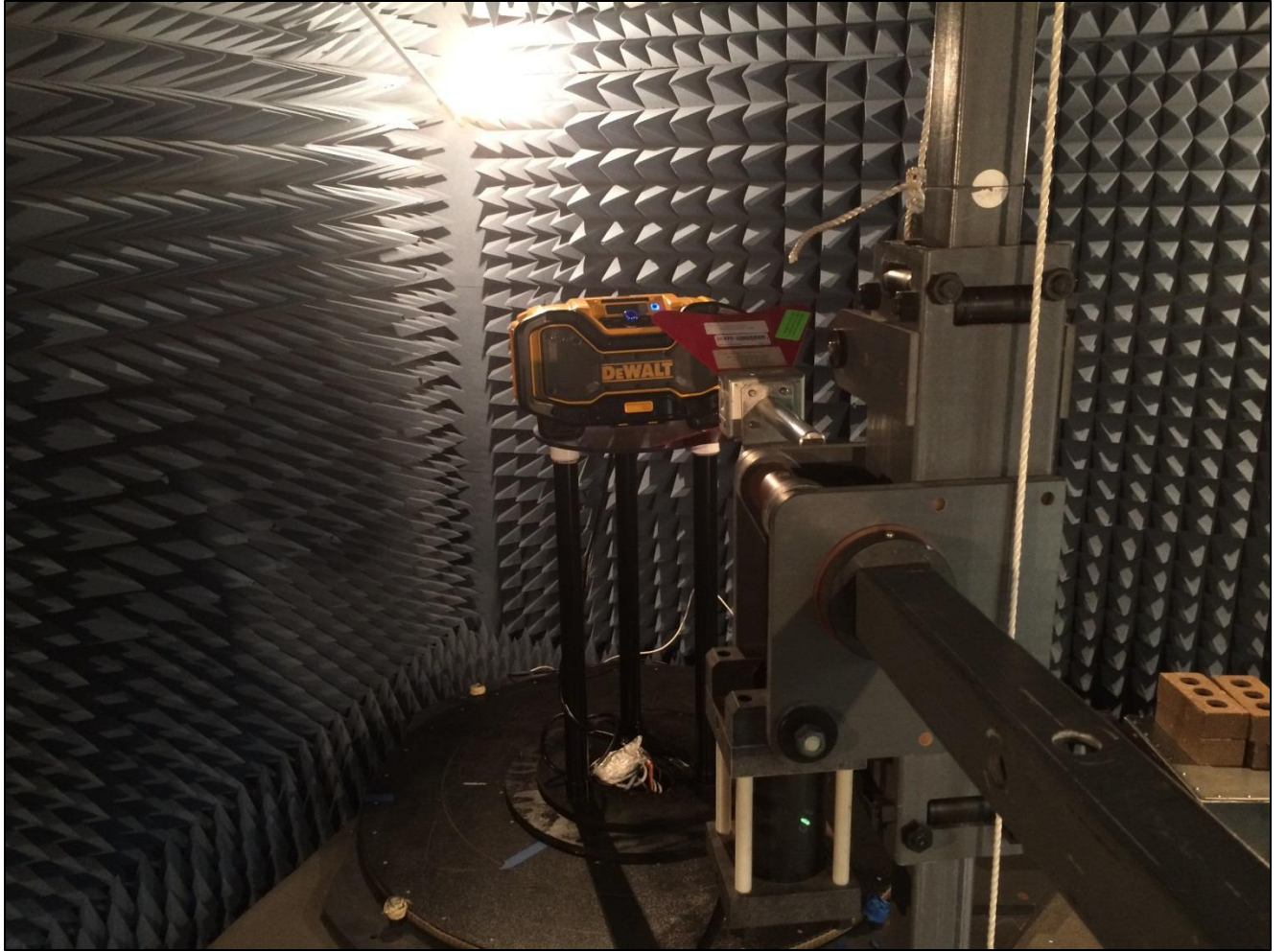
Photograph 3. Radiated Spurious Emissions, Test Setup Above 1 GHz
