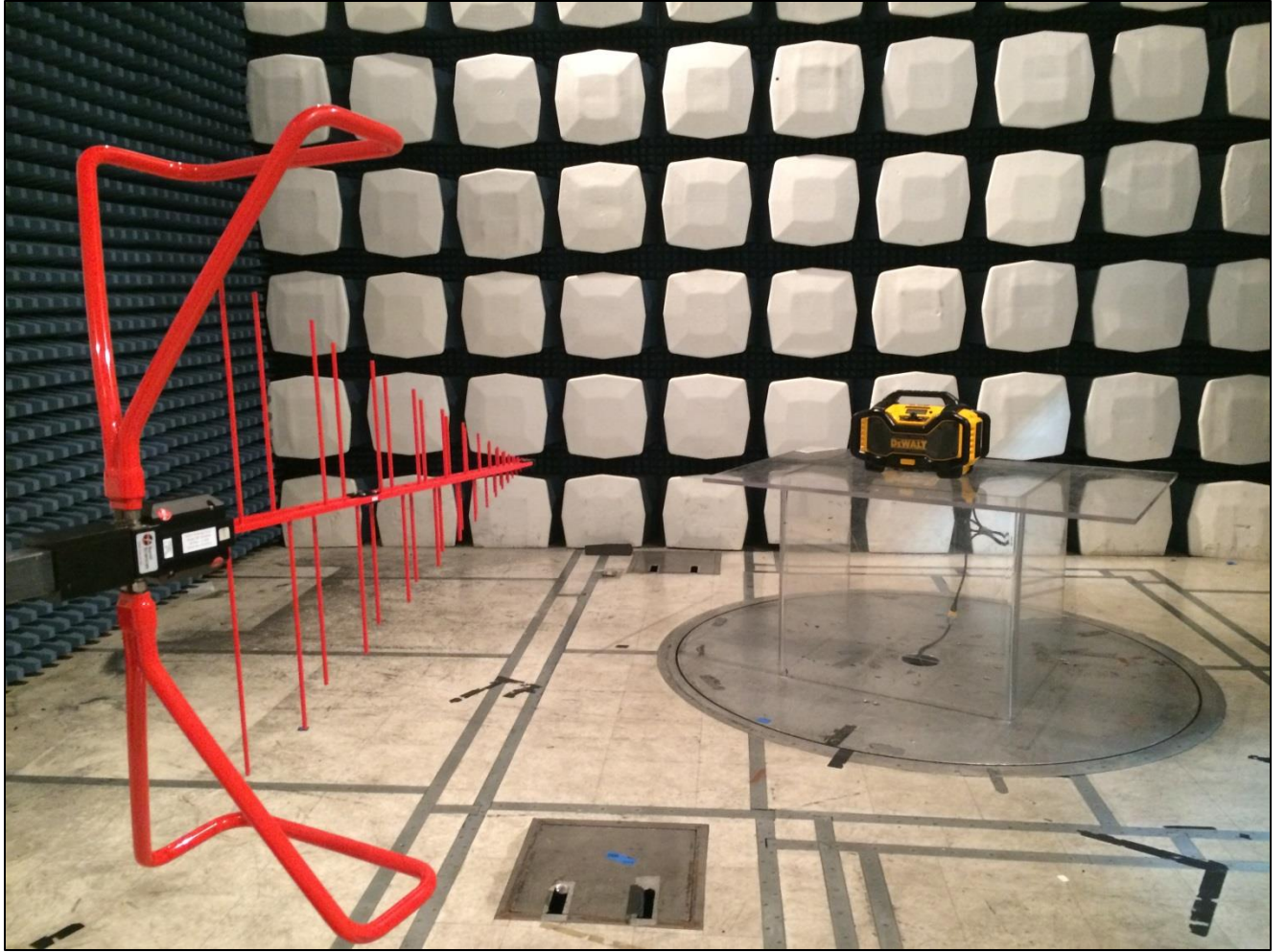
Photograph 2. Radiated Spurious Emissions, Test Setup Below 1 GHz
