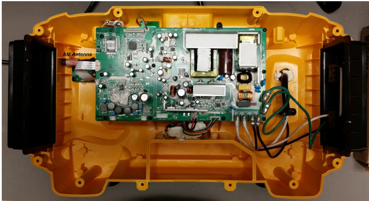
Photograph 2. DCR025_Inside_Radio_Shields_Removed
