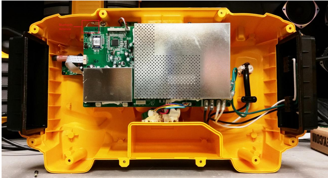
Photograph 3. DCR025_Inside_Radio_Shields_Still_On BT Ant
