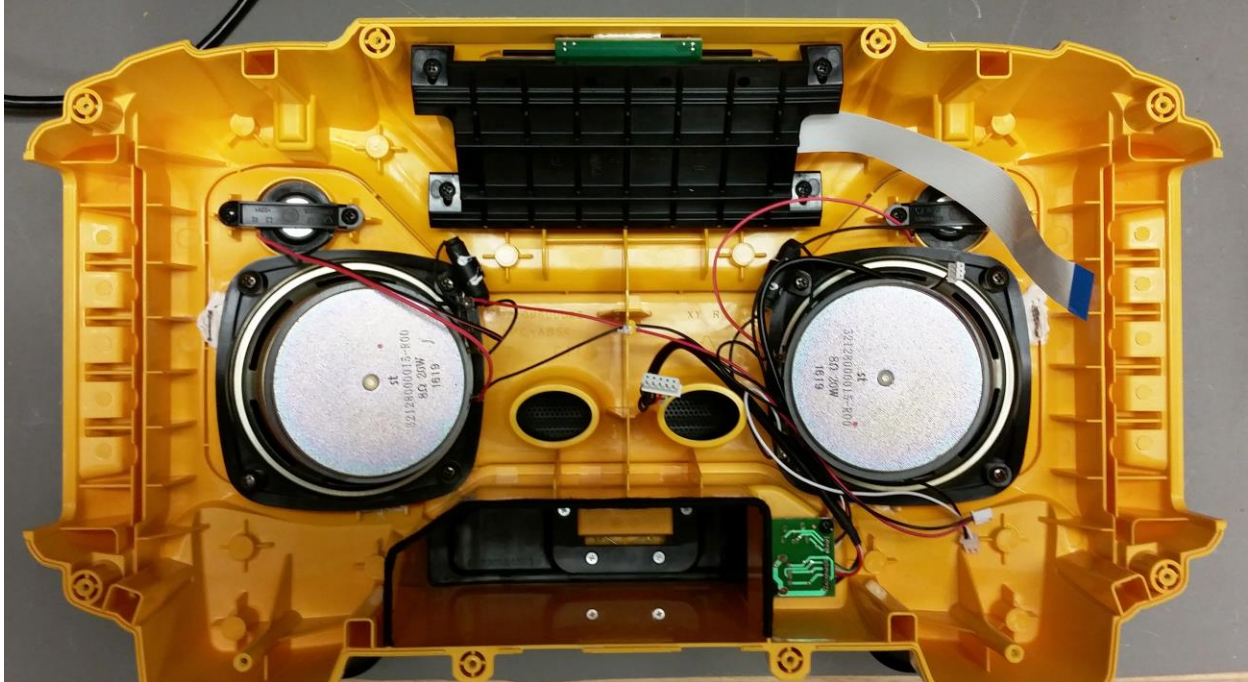
Photograph 5. DCR025_Inside_Speakers
