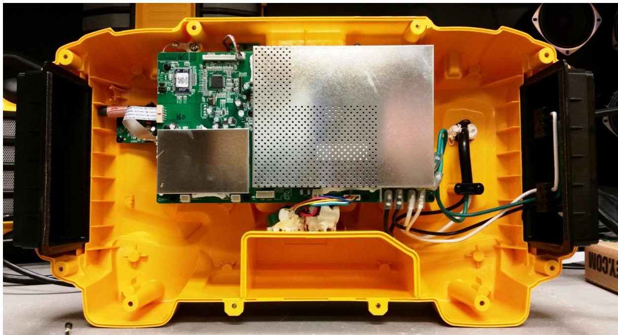
Photograph 4. DCR025_Inside_Radio_Shields_Still_On
