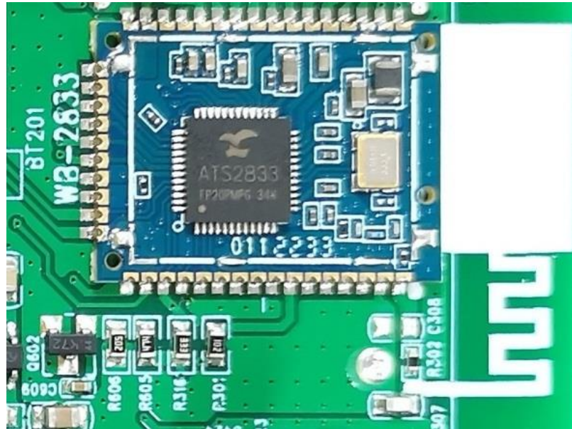
Figure 2: Antenna on the PCB
