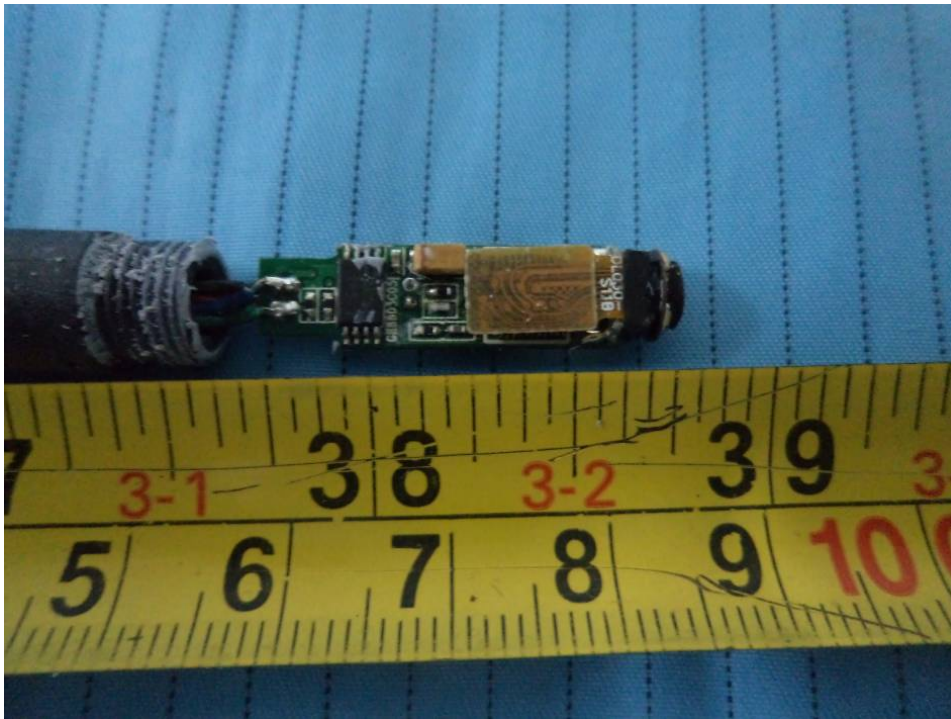
EUT –Tube Board Bottom View
