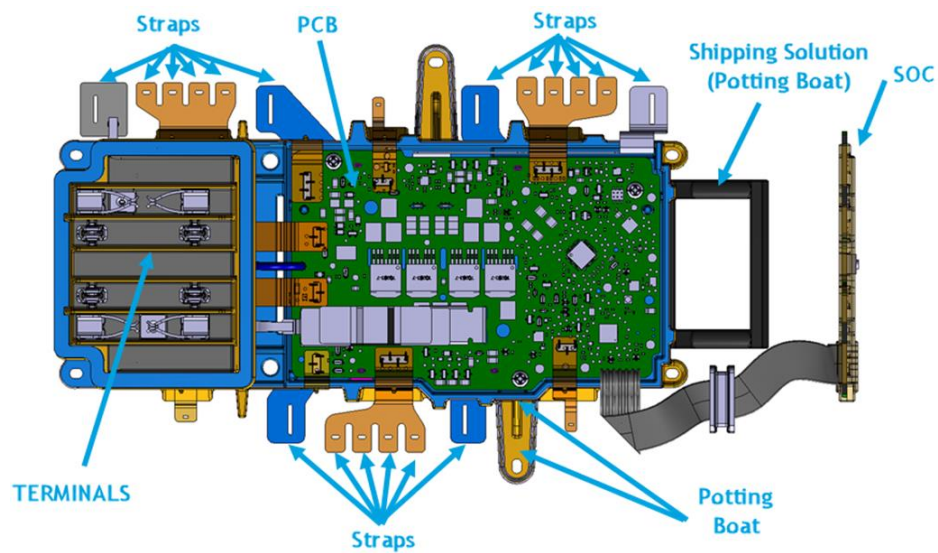
Figure 1: NA382408 Assembly
