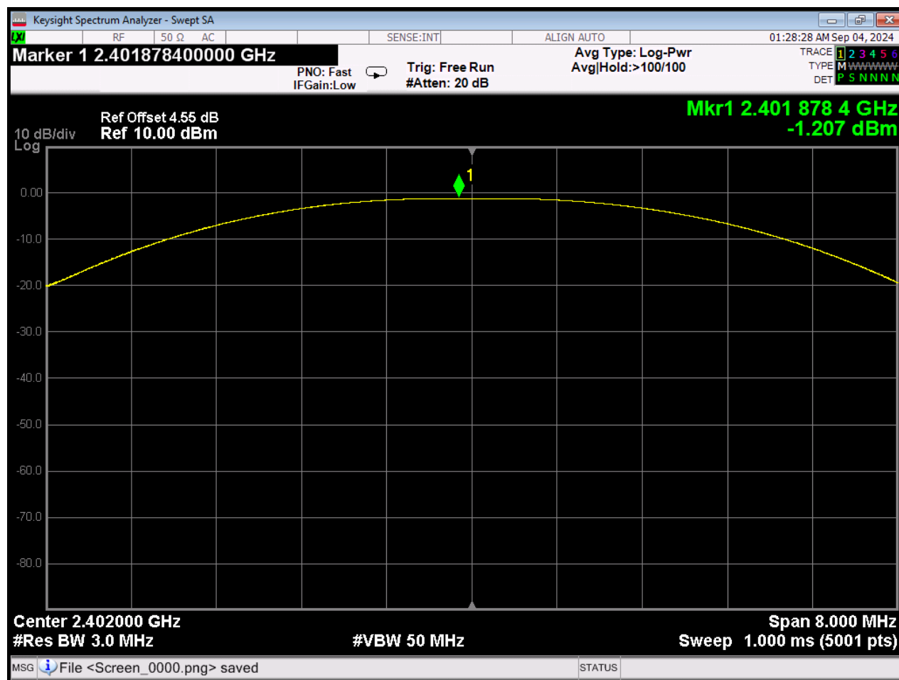
Figure 4: CIIPC, Peak Transmit Power, 1Mbps (DH5) (Conducted, Antenna Port)
