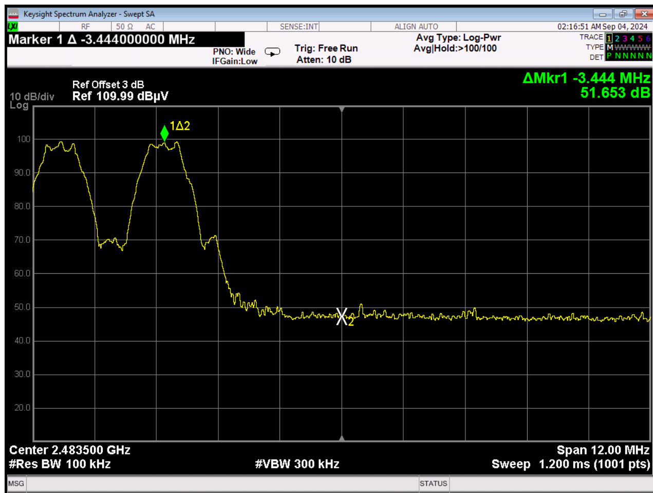
Figure 9: CIIPC, Worst-Case Band-Edge, High Channel
