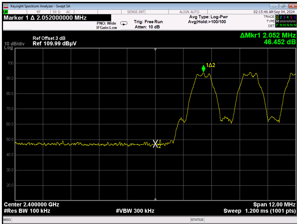
Figure 8: CIIPC, Worst-Case Band-Edge, Low Channel
