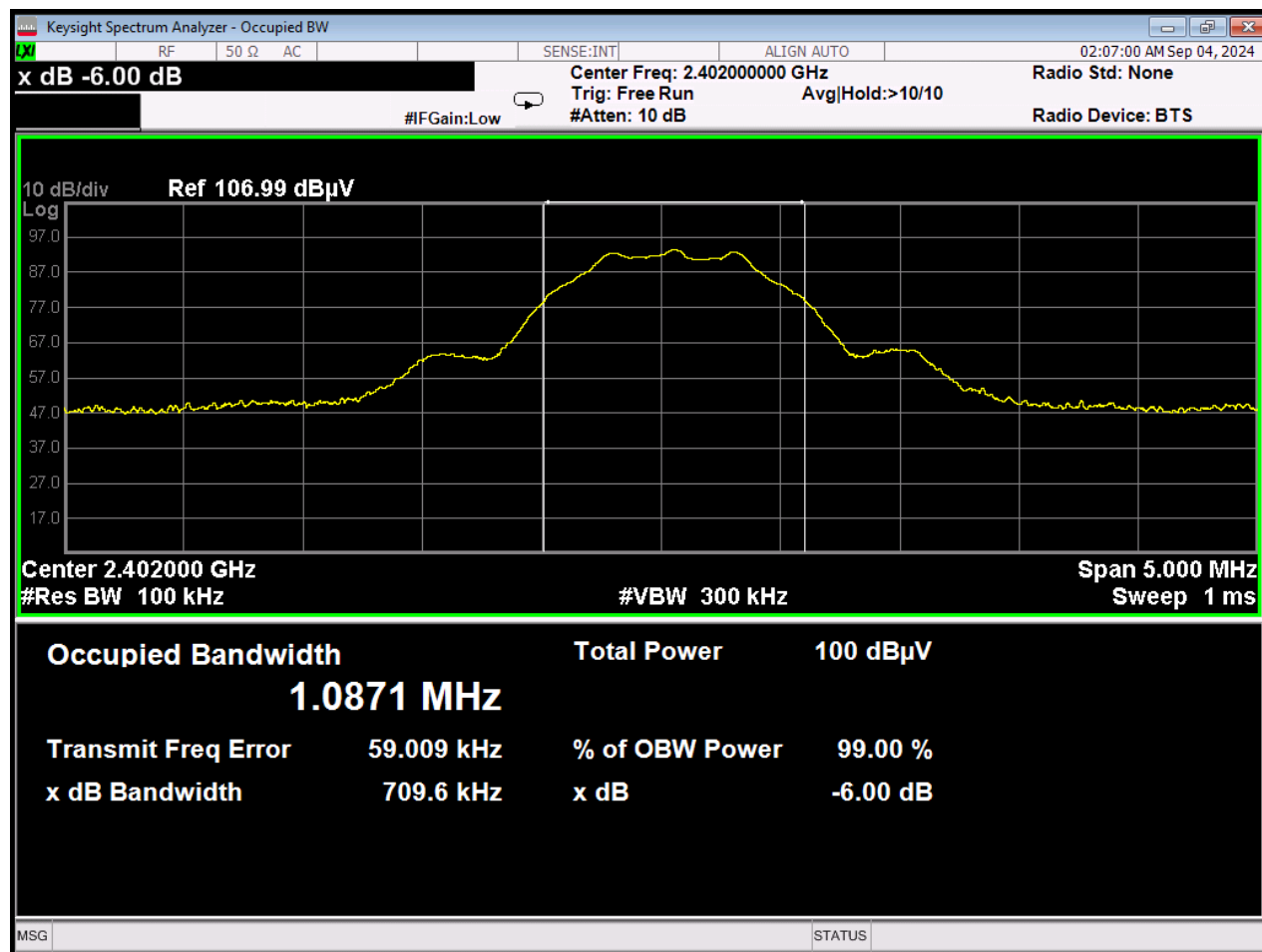
Figure 3: CIIPC Occupied Bandwidth, Low Channel, 1Mbps
