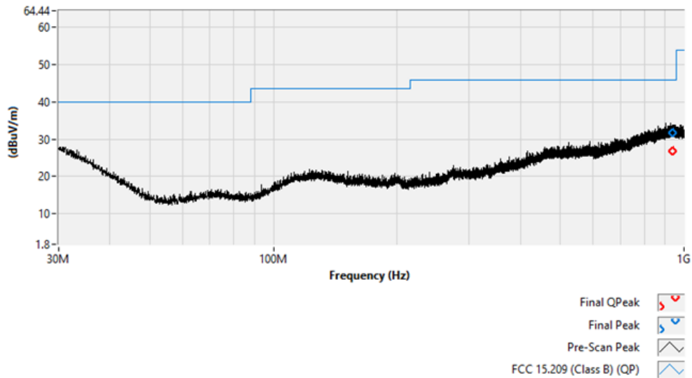
Worst-Case Pre-scan and Final Data (Horizontal)
