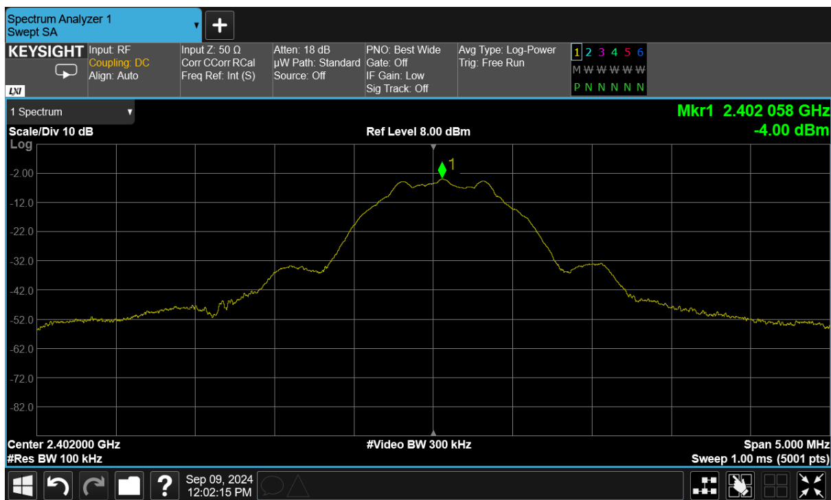
Figure 6: CIIPC Power Spectral Density, Low Channel, 1Mbps (DH5) (Conducted, Antenna Port)
