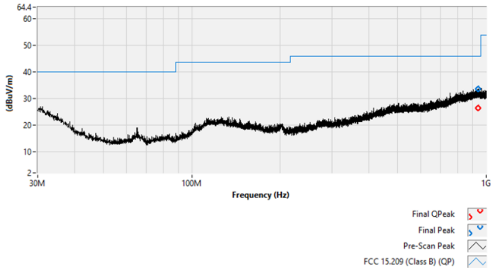
Worst-Case Pre-scan and Final Data (Vertical)
