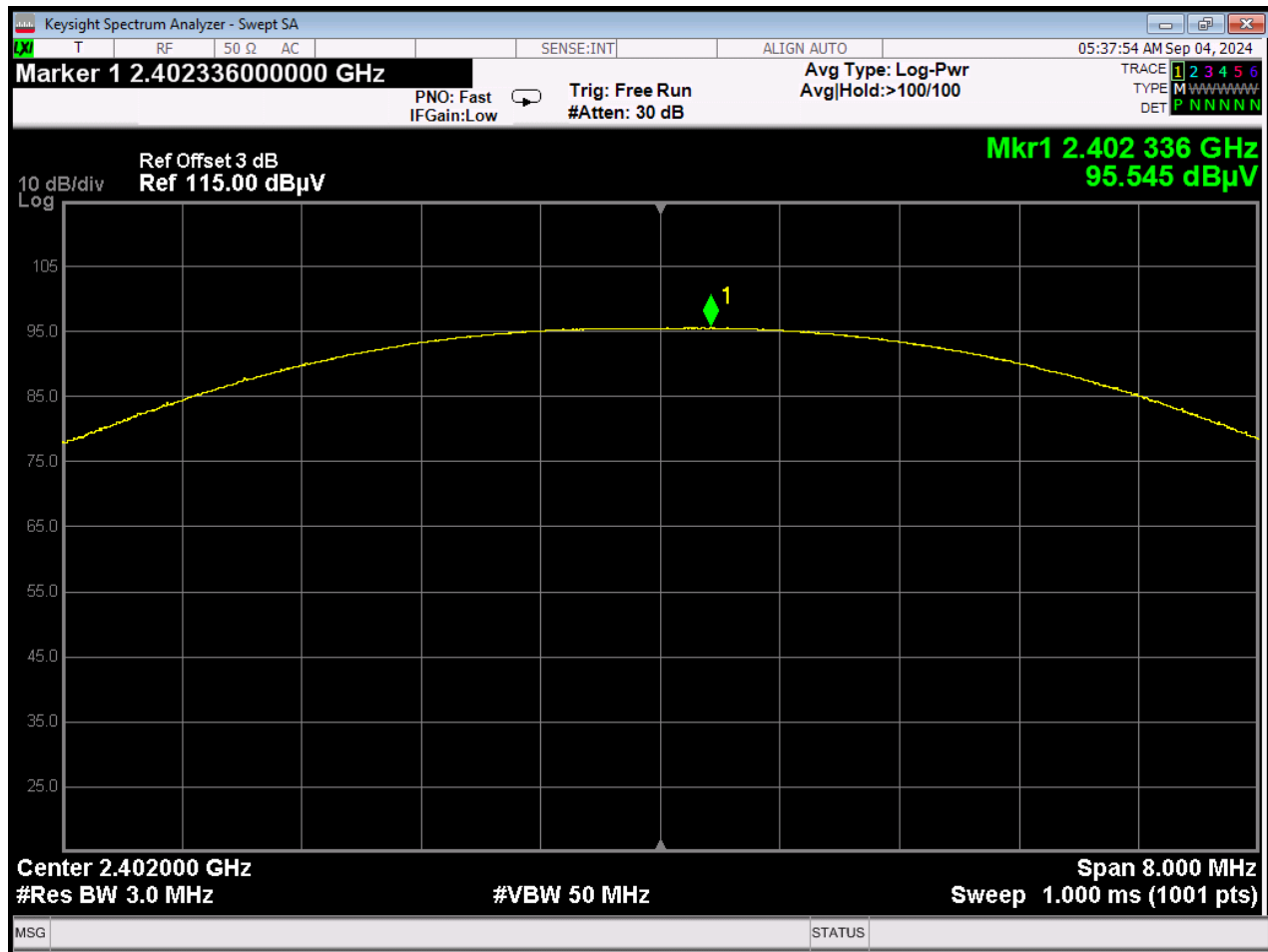
Figure 5: CIIPC, Radiated Power, 1Mbps (DH5) (3-meter Radiated)
