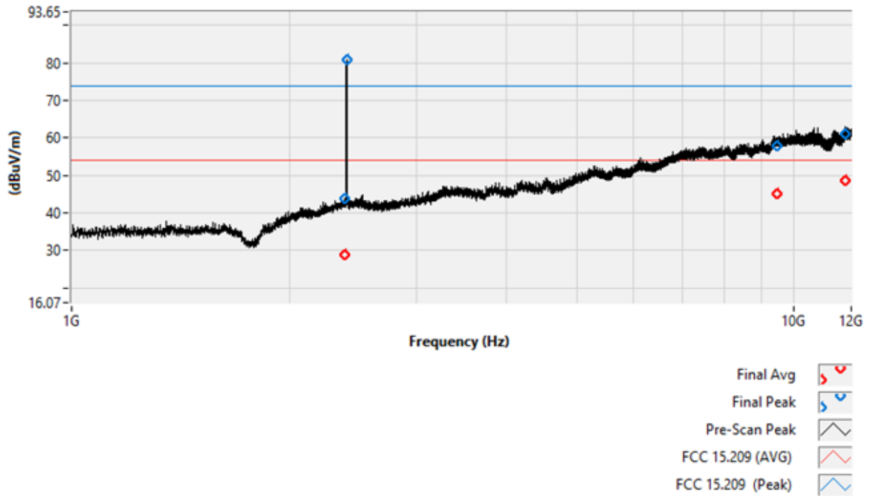
Worst-Case Pre-scan and Final Data (Vertical)
