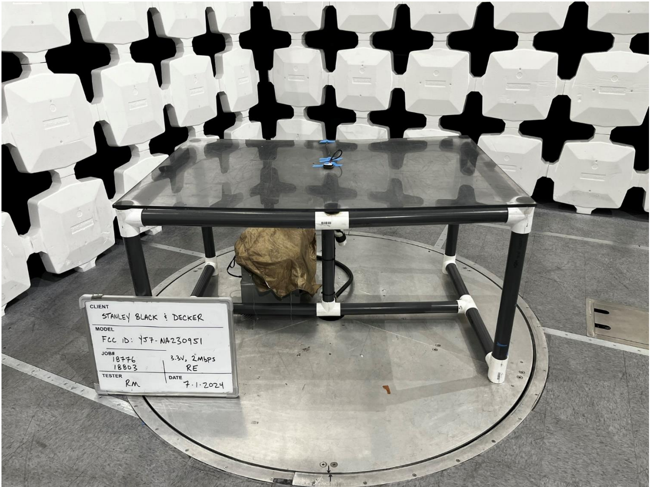
3-meter Radiated Emission, Front View #2 (30M-1GHz)
