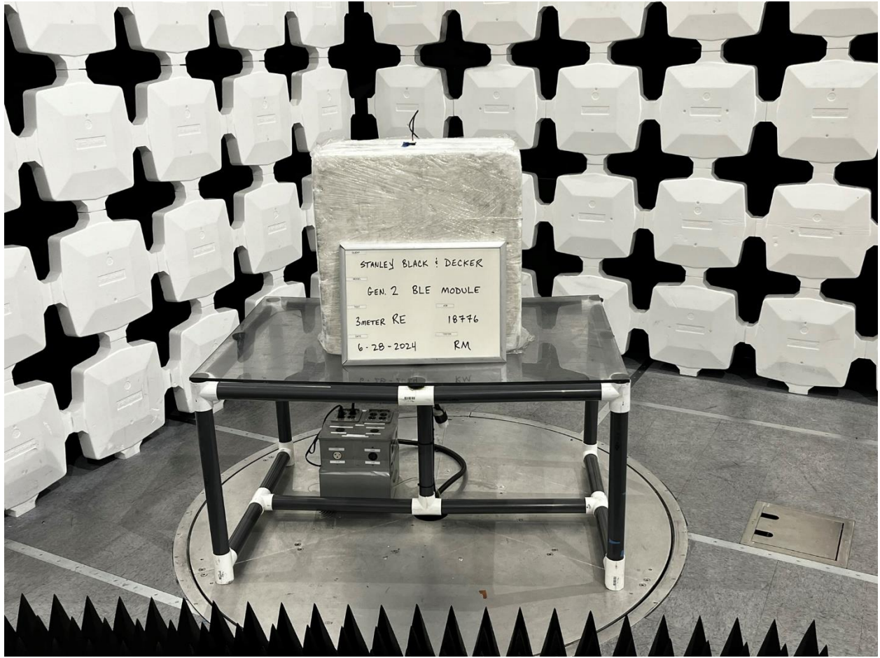
3-meter Radiated Emission, Front View #1 (Above 1GHz)
