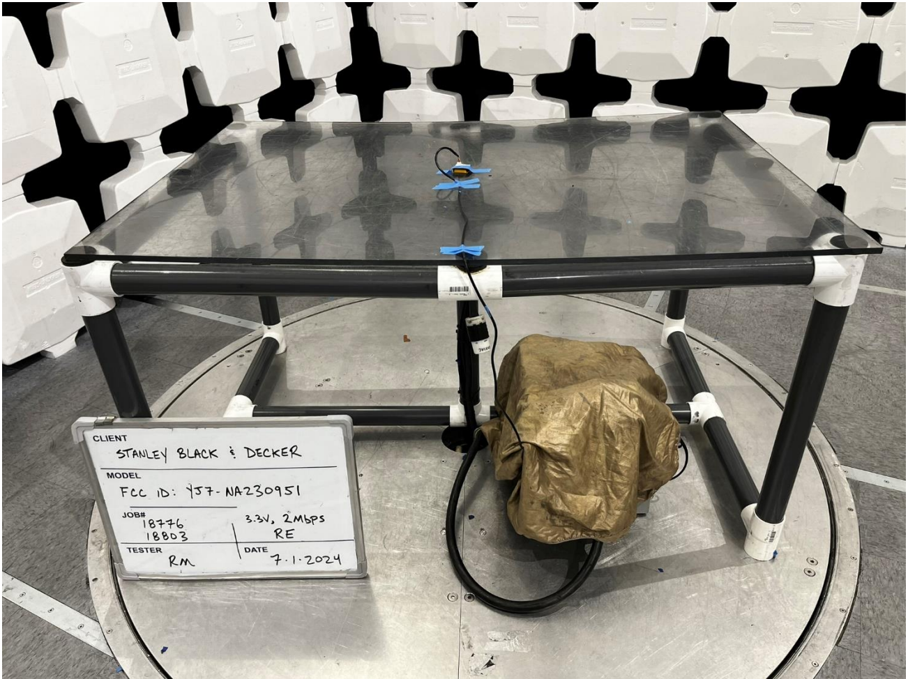
3-meter Radiated Emission, Rear View #2 (30M-1GHz)
