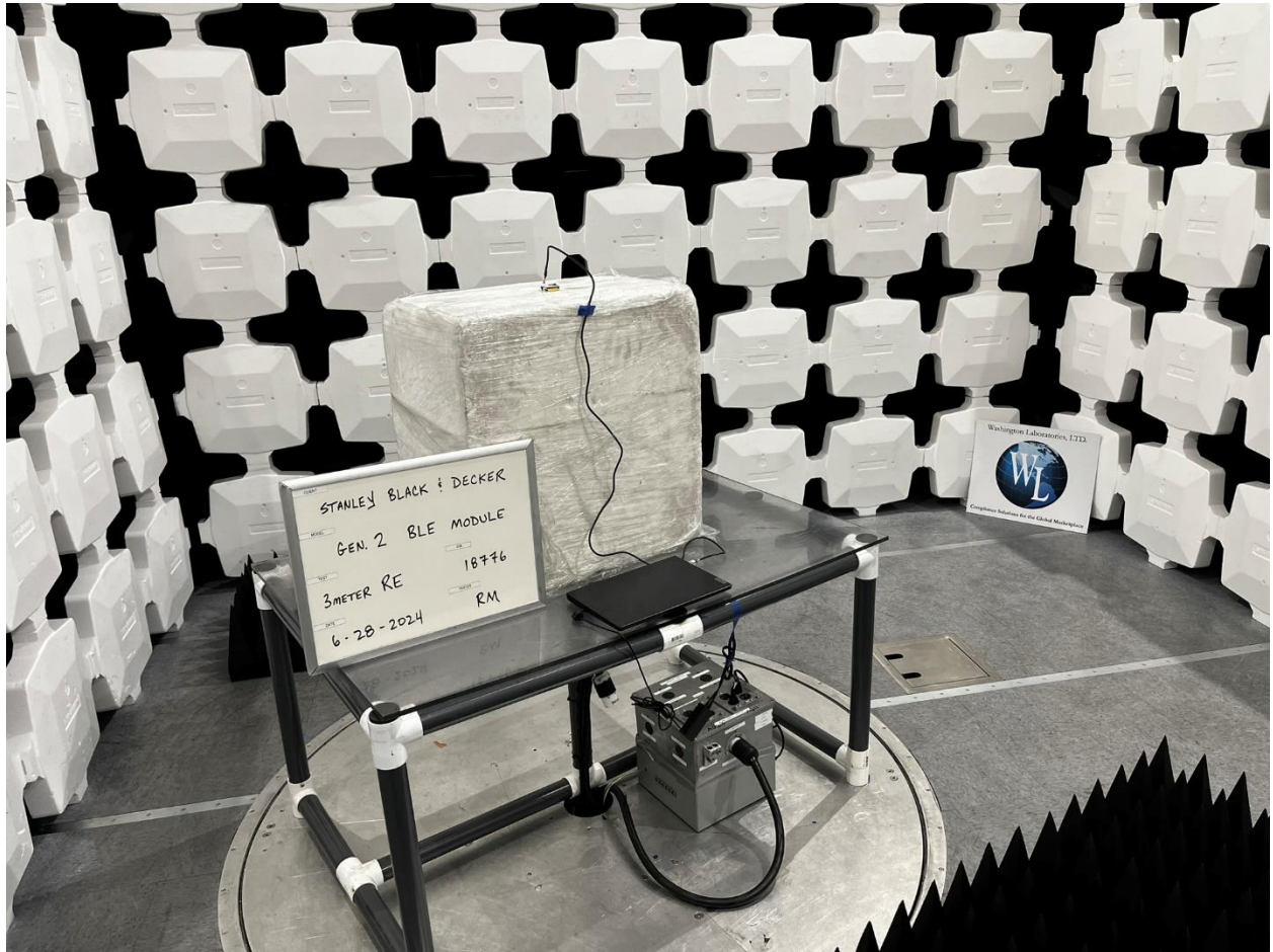
3-meter Radiated Emission, Rear View #1 (Above 1GHz)
