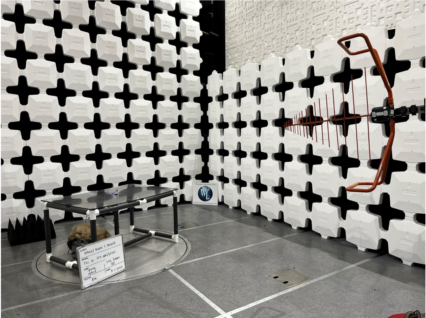
3-meter Radiated Emission, Front View #1 (30M-1GHz)
