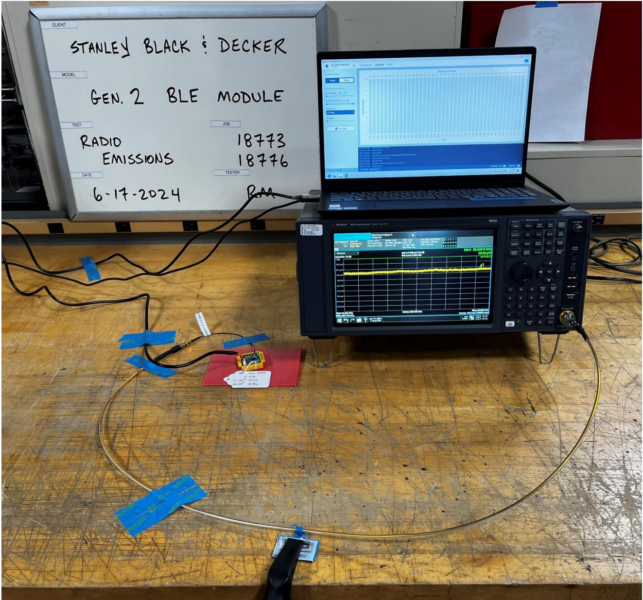
Benchtop Conducted, Radio Emissions
