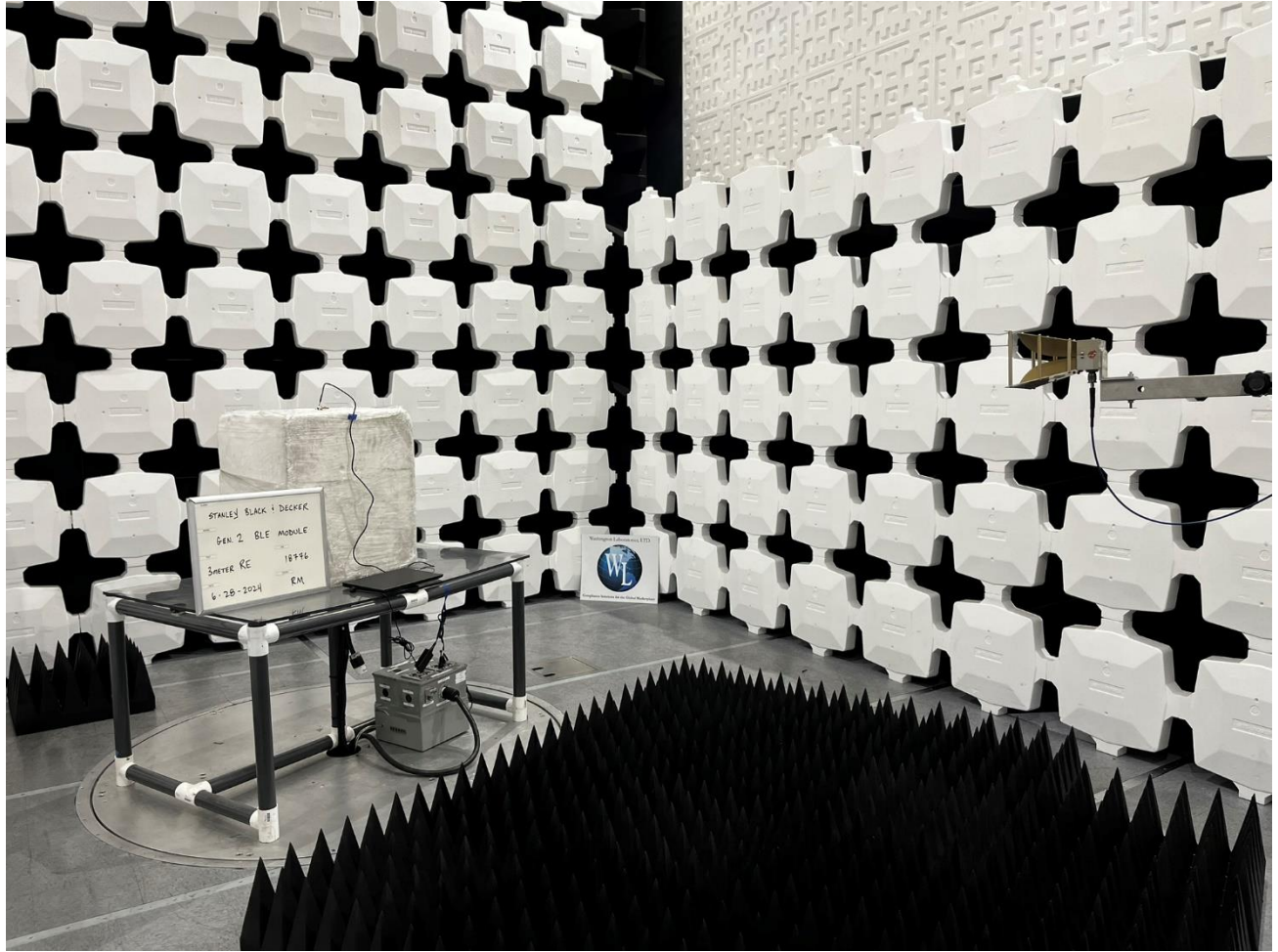
3-meter Radiated Emission, Front View #2 (Above 1GHz)
