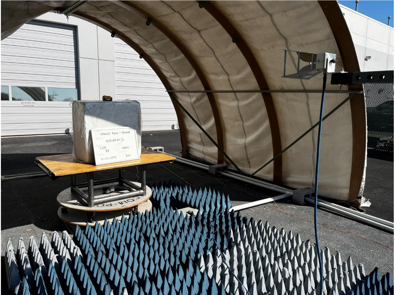
Radiated Emissions View 3, >1GHz
