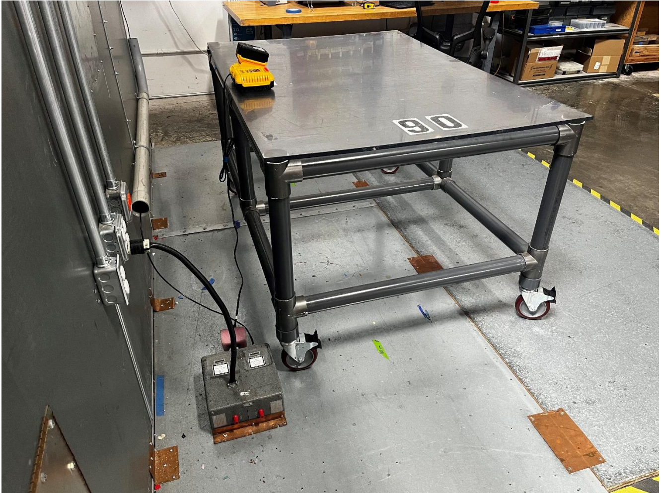
AC Powerline Emissions Side View
