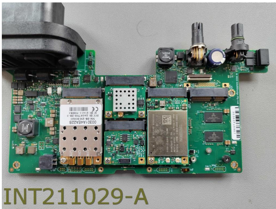
Base PCB – Top View
