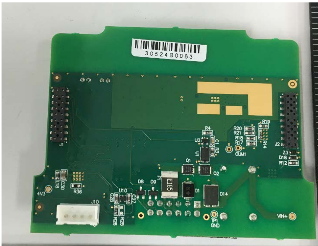
PCB_1 – Bottom
