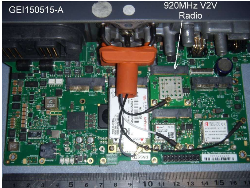
PROD0847-2 – Main Board (showing 920MHz V2V Radio)
