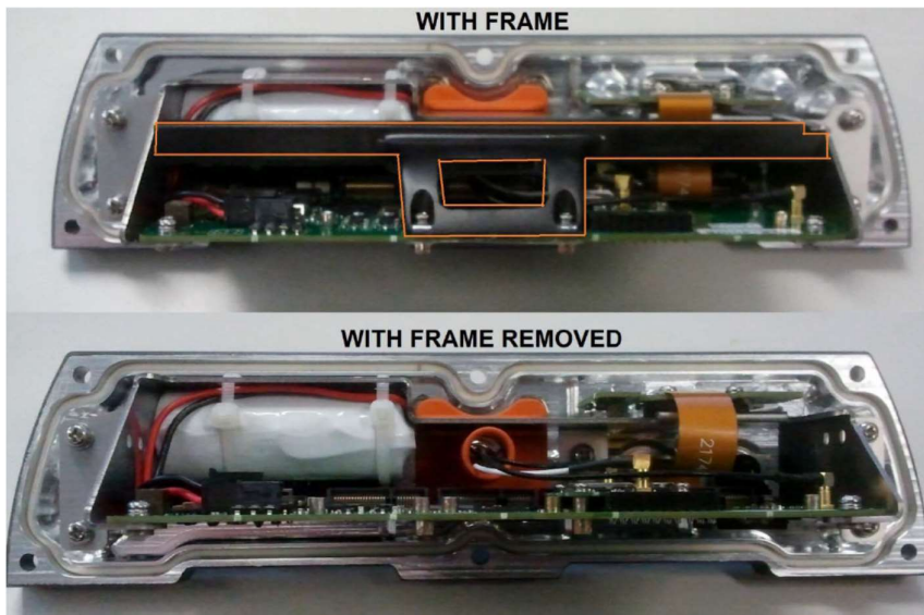
PROD0847-2 – IVU Frame
