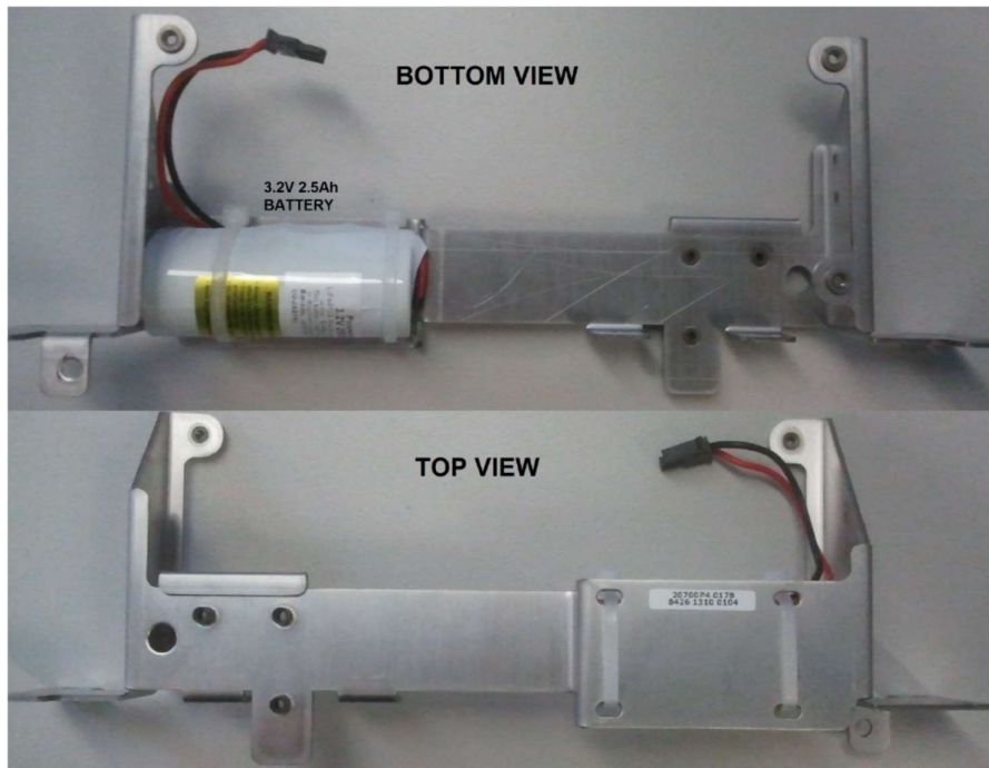
PROD0847-2 – IVU Chassis
