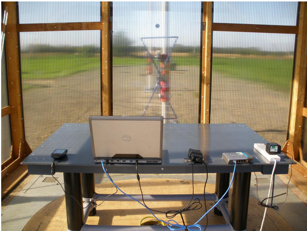
Photograph 4 Radiated Emissions - Connected to PC - Back
