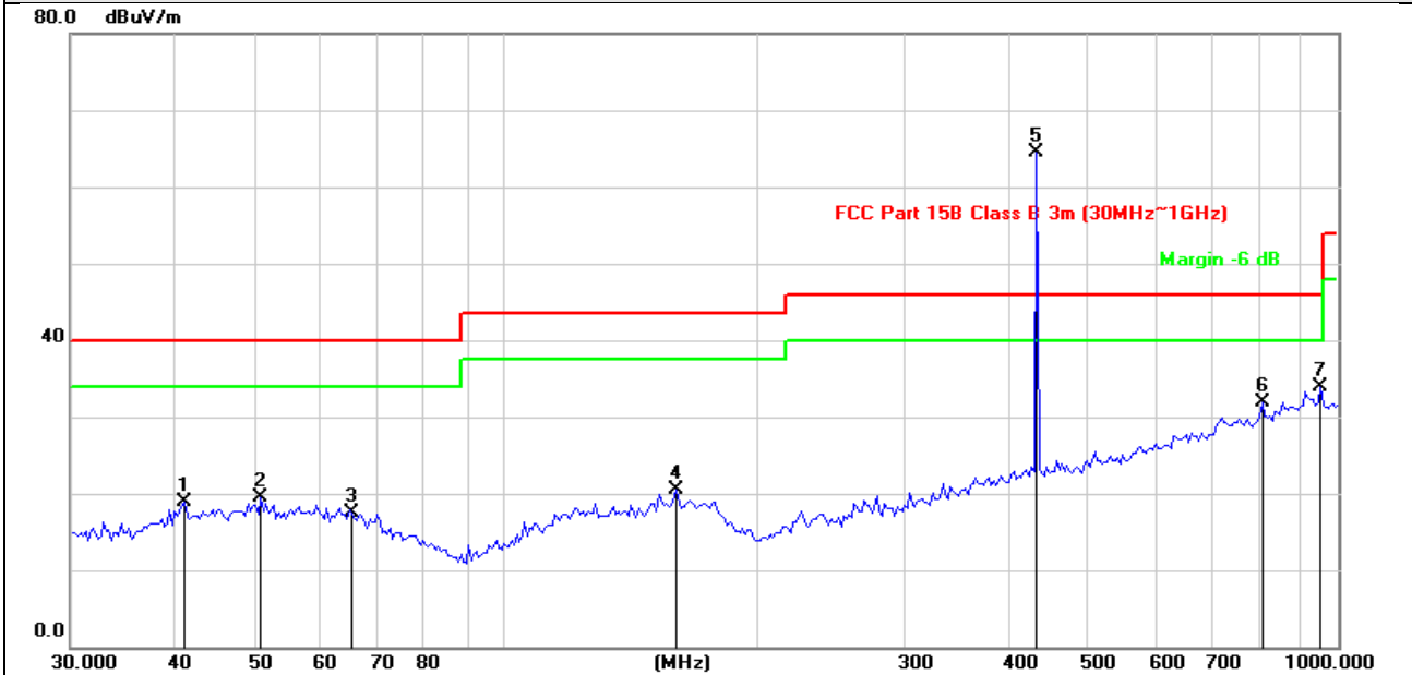
Antenna Polarity & Test distance: Vertical at3m
