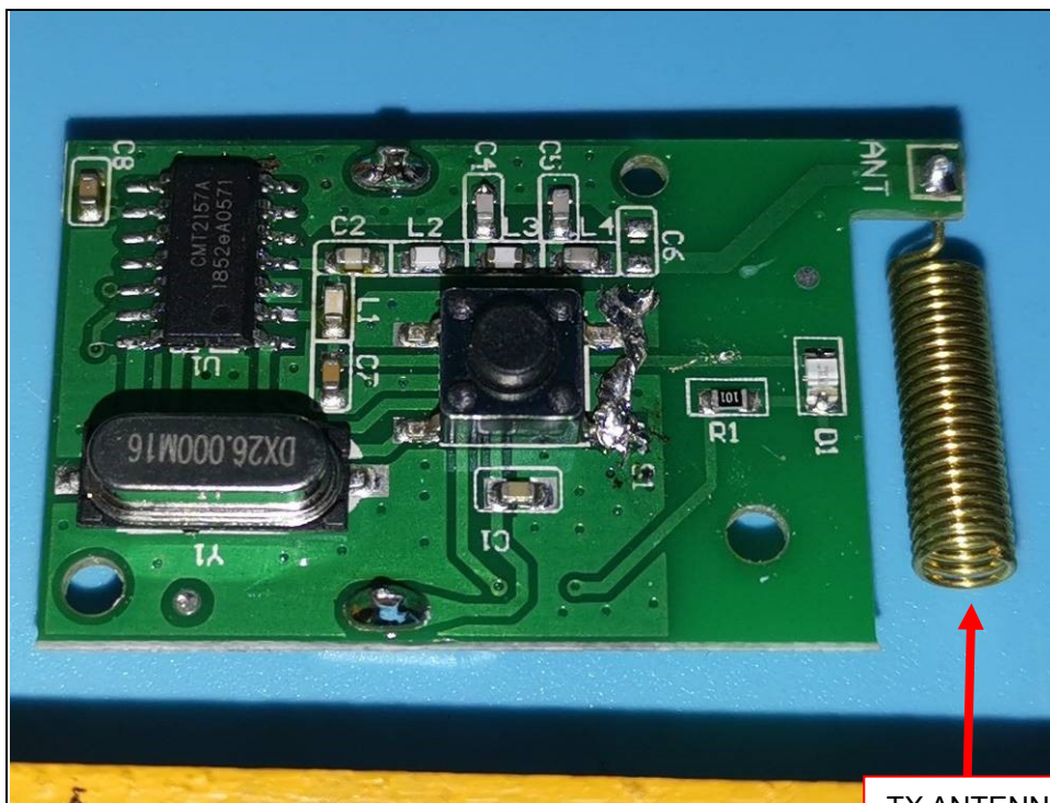
TX ANTENNA
