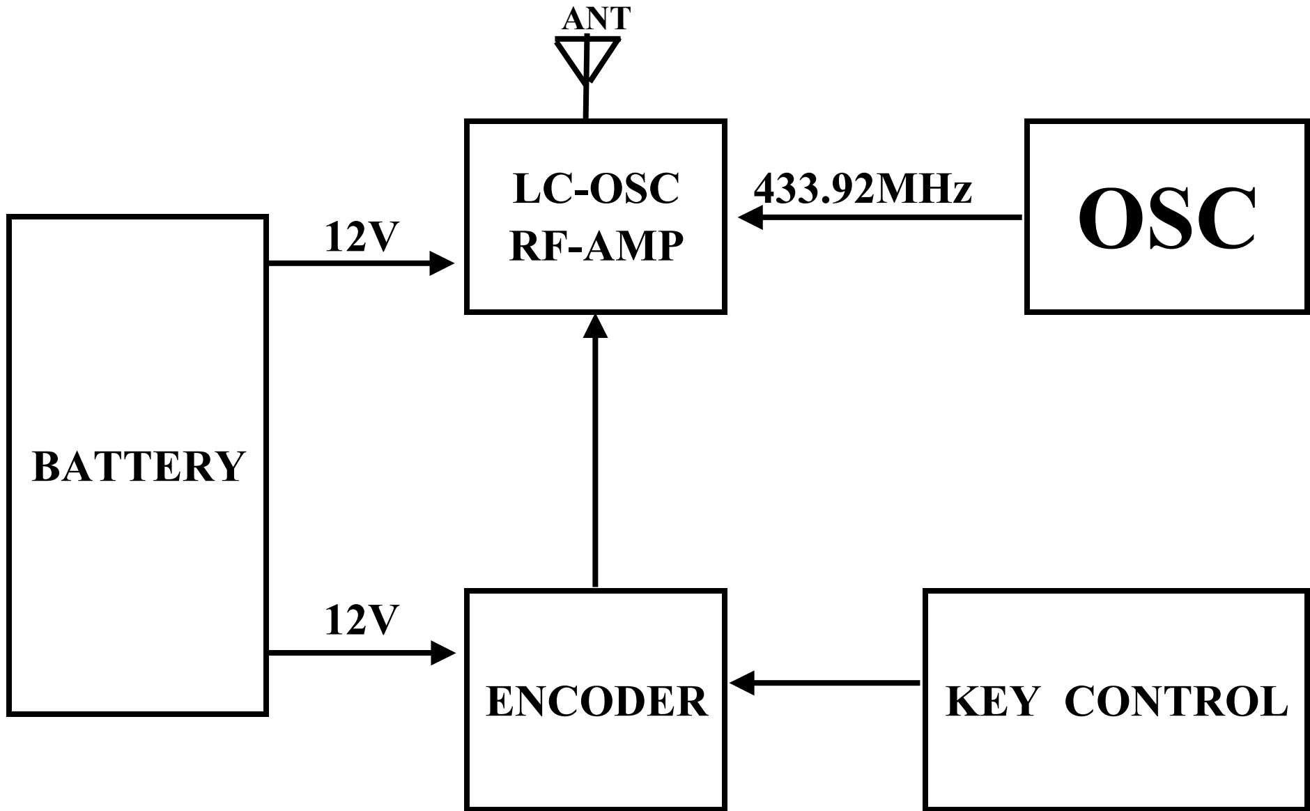
RL-0507A TRANSMITTER BLOCK(TR SYS)
