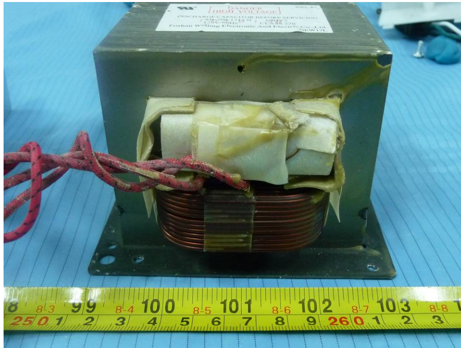
EUT – Power Transformer Side View
