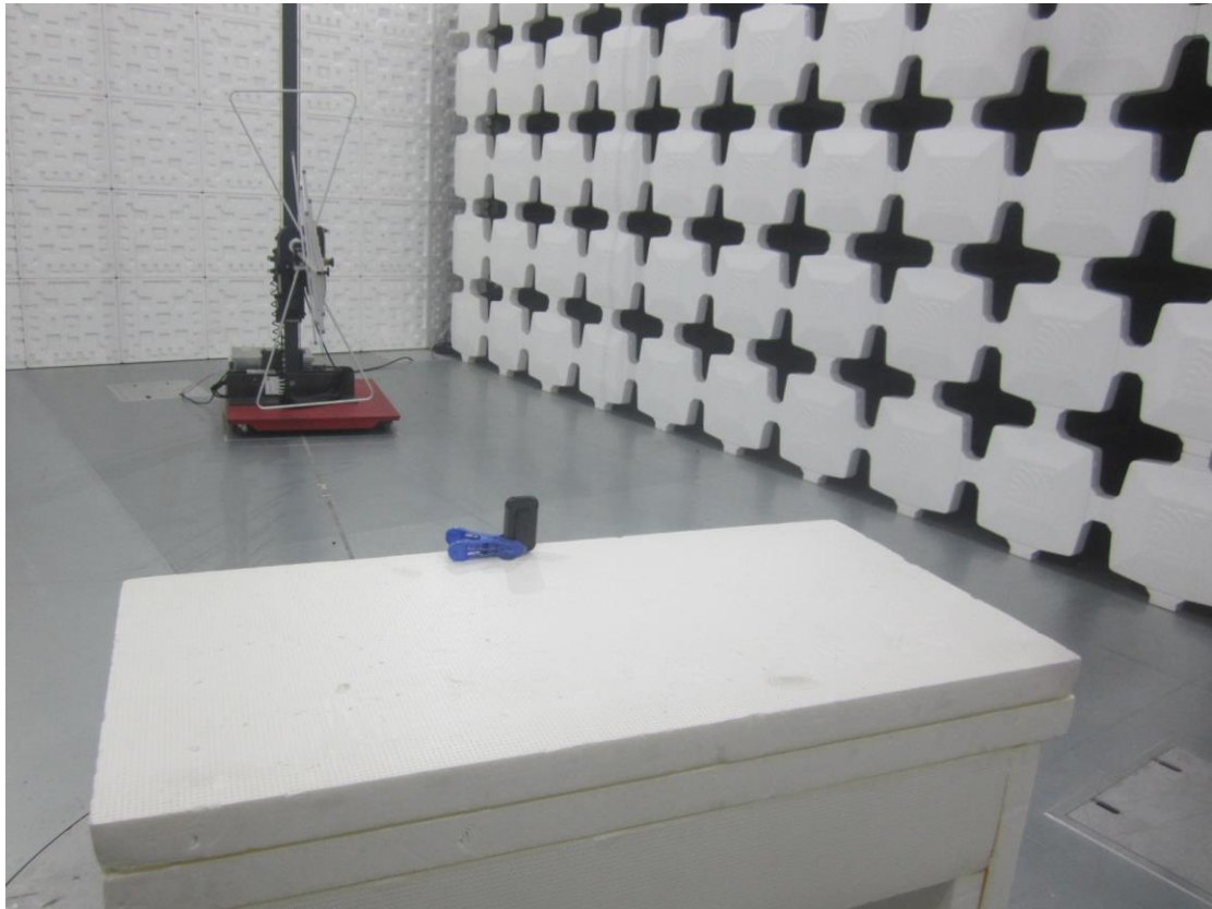
Radiated Emission (30MHz-1000MHz)
