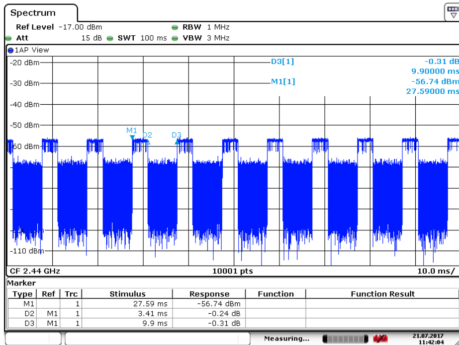
Remote Controller 2440MHz
