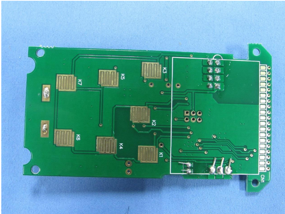
PCB view of remote controller
