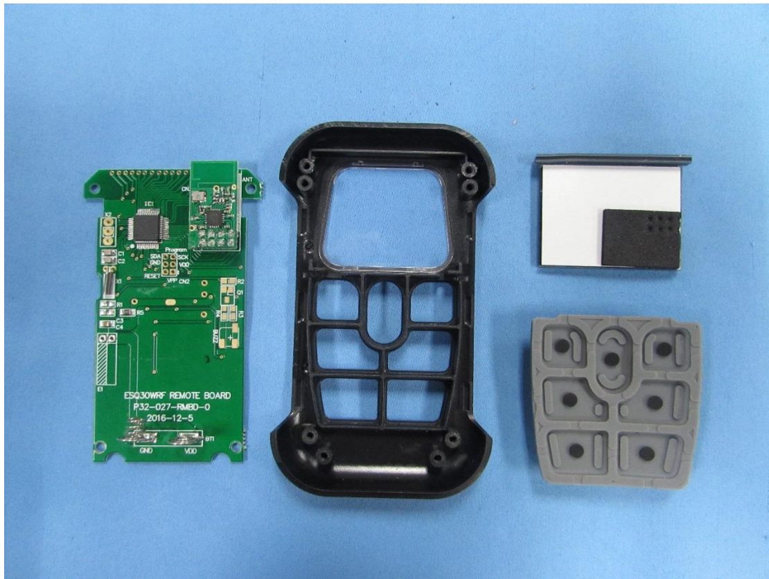
Internal view of remote controller
