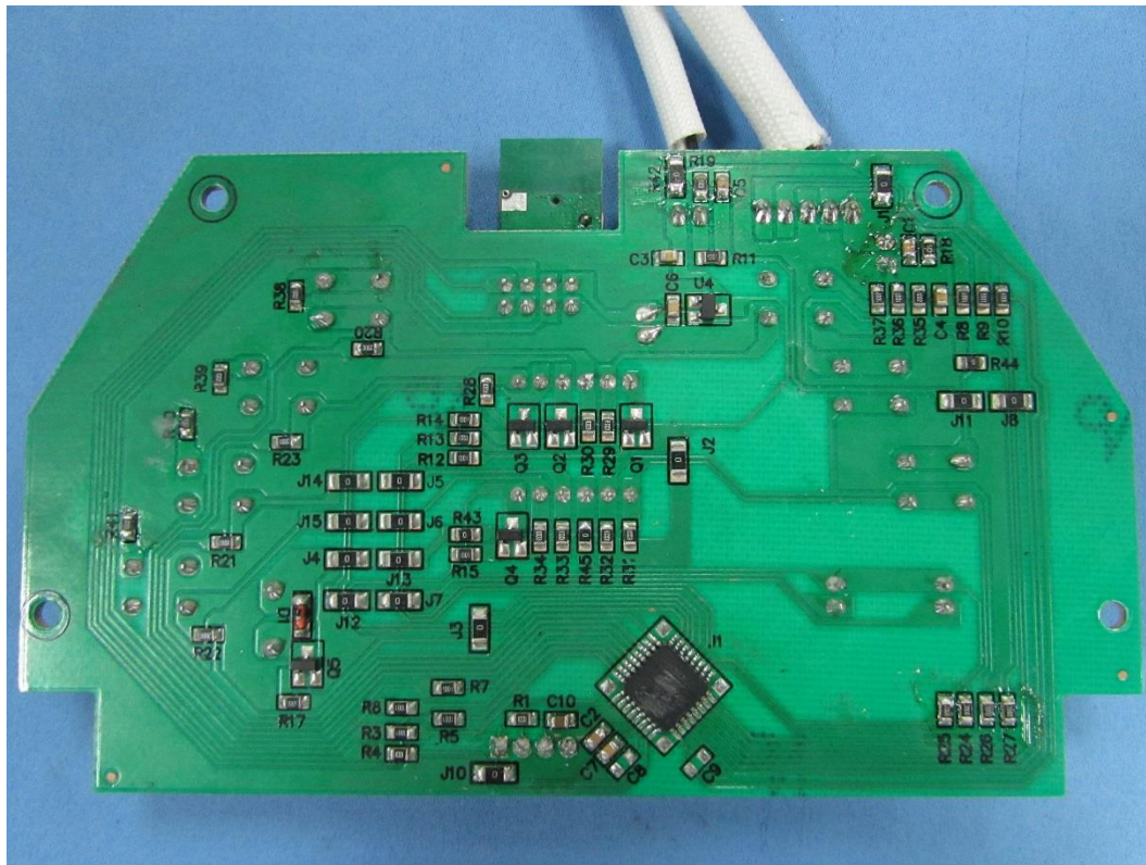
PCB view of controller
