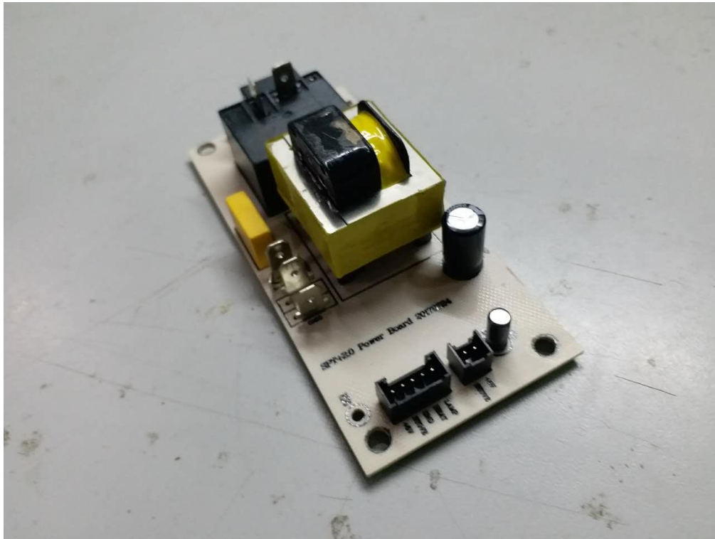
PCB view of power board of smoker
