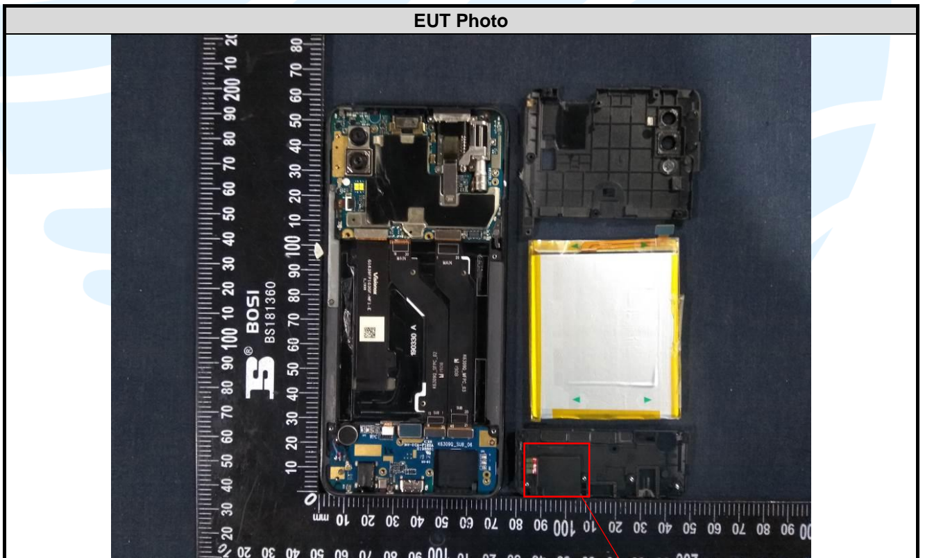
2/3/4G Antenna
