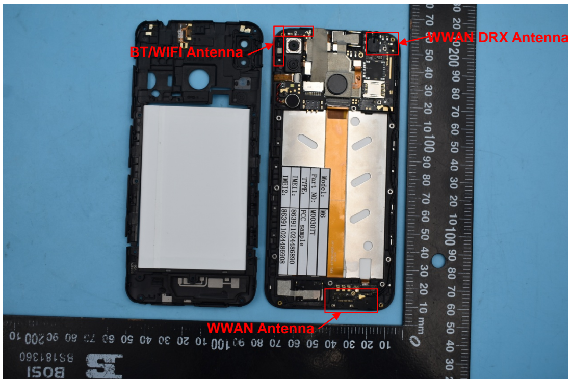
2. Antenna view
