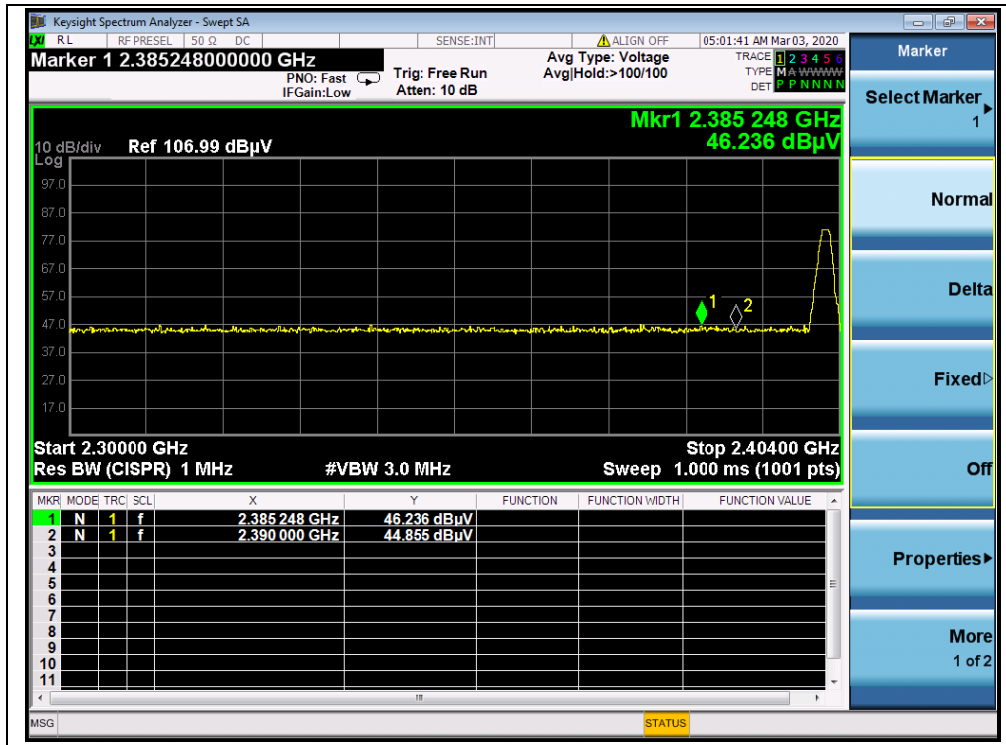
(Channel = 0, PEAK)
