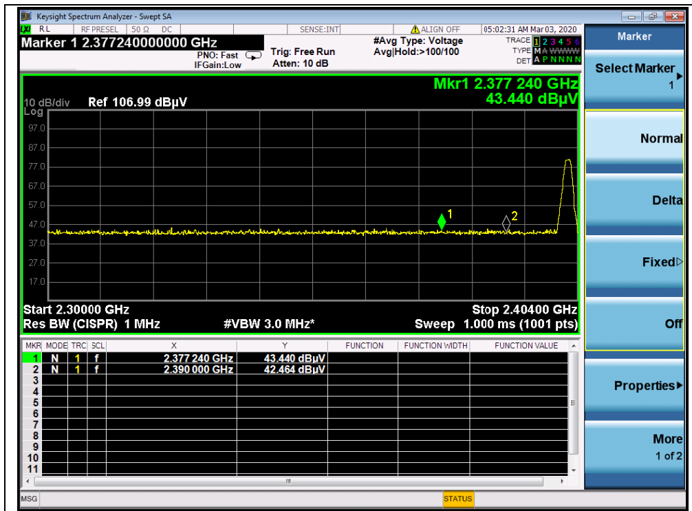
(Channel = 0, AVG)
