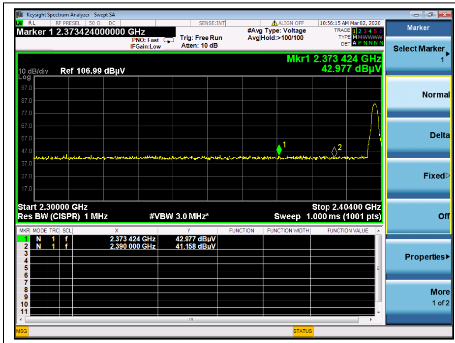
(Channel = 0, AVERAGE, GFSK)
