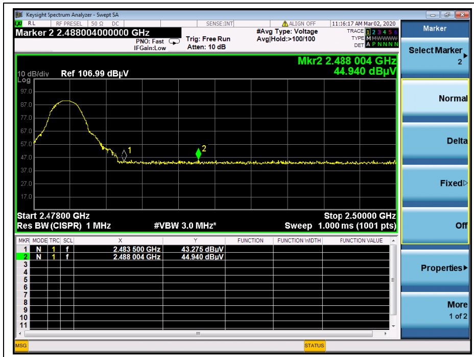
(Channel = 78, AVERAGE, GFSK)
