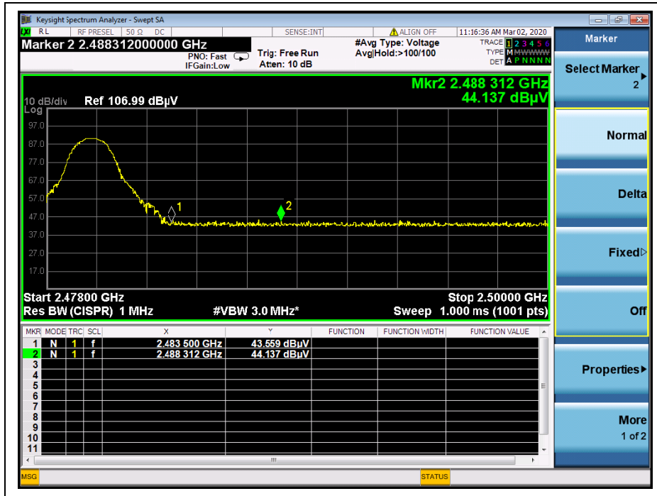
(Channel = 78, AVERAGE, \pi/4 -DQPSK)
