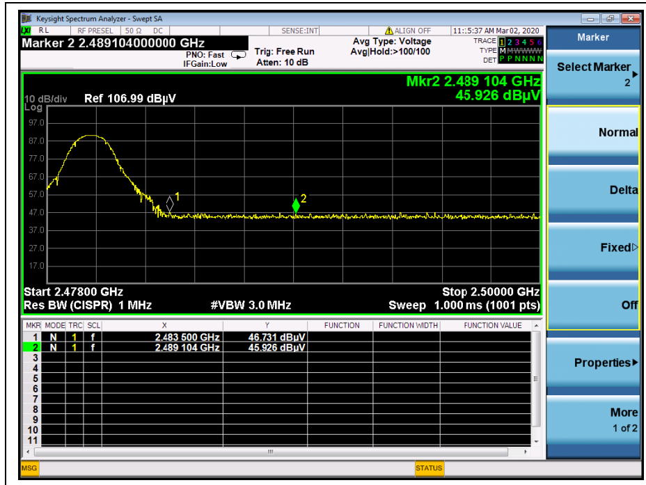
(Channel = 78, PEAK, GFSK)
