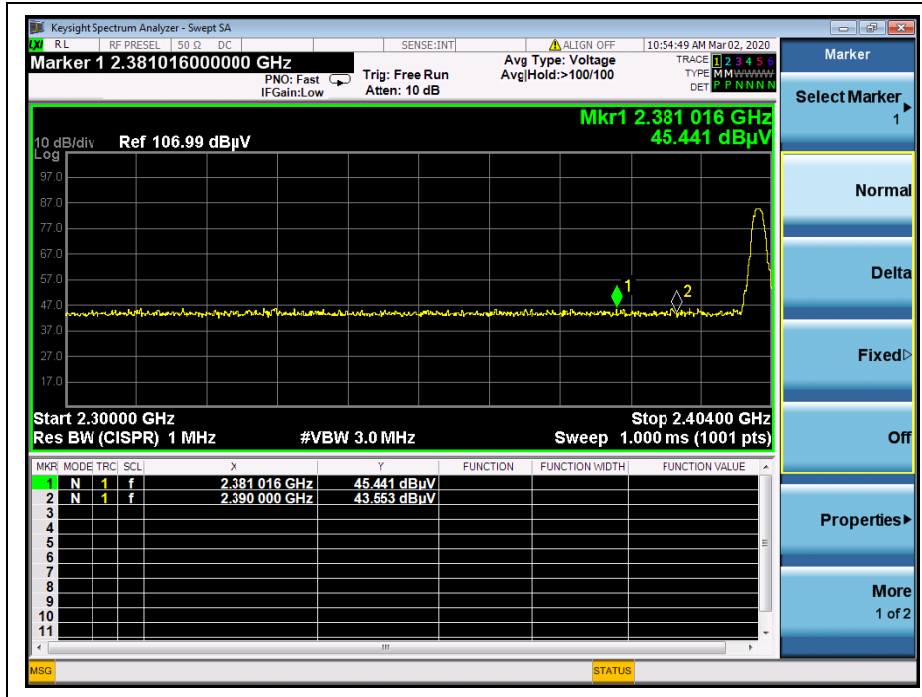
(Channel = 0, PEAK, GFSK)
