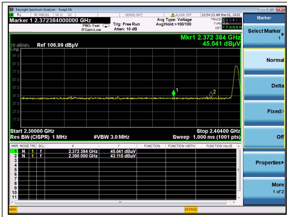
(Channel = 0, PEAK, \pi/4 -DQPSK)
