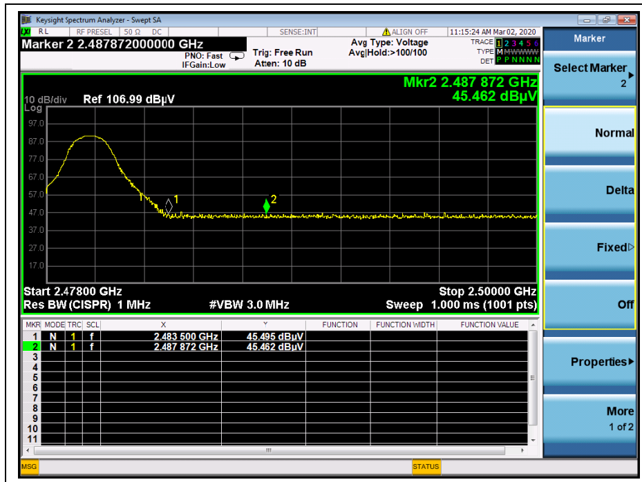
(Channel = 78, PEAK, \pi/4 -DQPSK)
