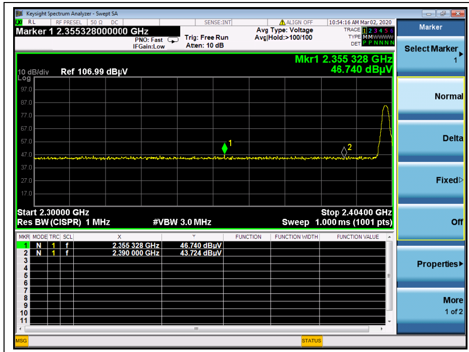
(Channel = 0, PEAK, 8-DPSK)
