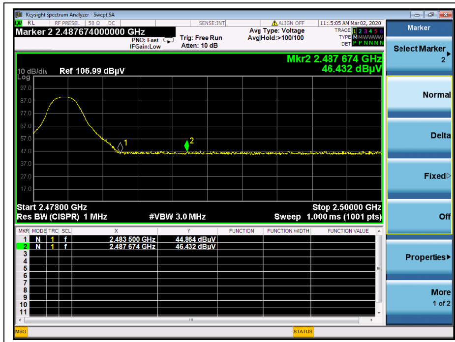
(Channel = 78, PEAK, 8-DPSK)
