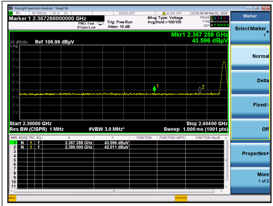
(Channel = 0, AVERAGE, \pi/4 -DQPSK)
