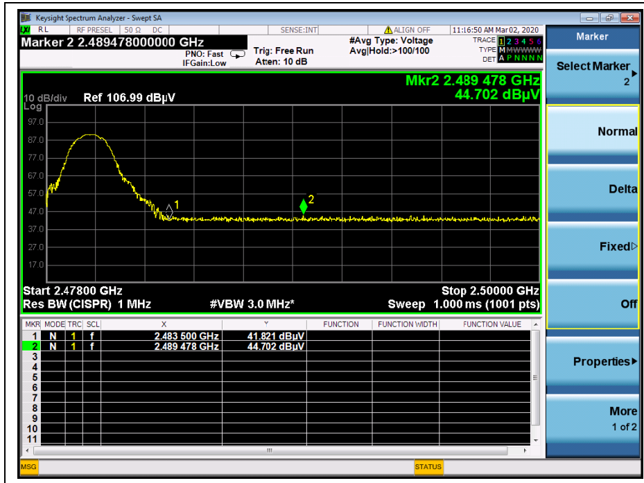
(Channel = 78, AVERAGE, 8-DPSK)
