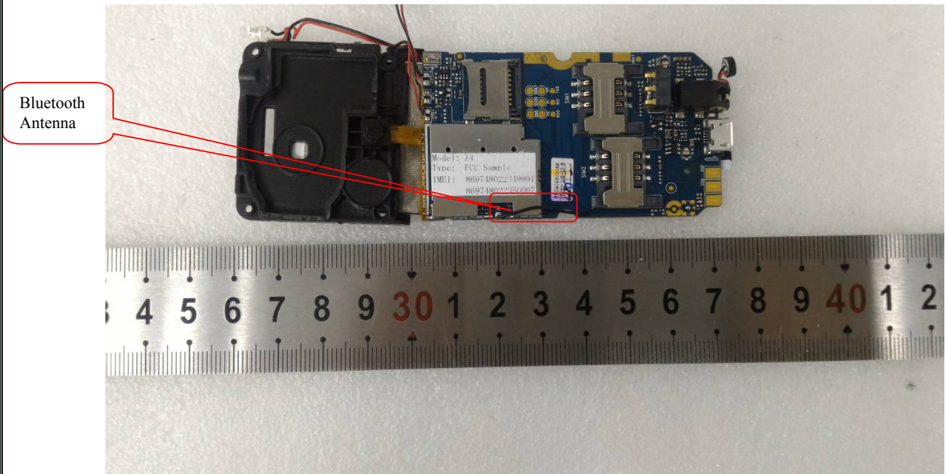
EUT – Mainboard Top View 1
