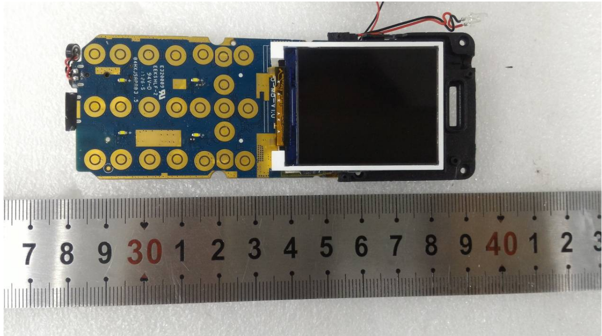
EUT – Mainboard Bottom Cover off View 2
