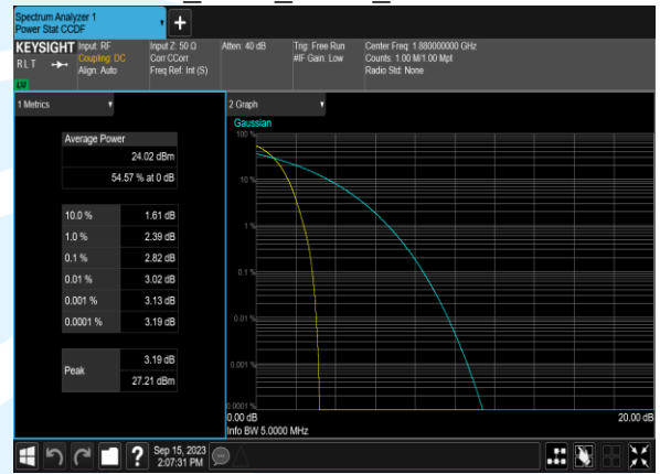
Band2_RMC_12.2k_Channel9400
