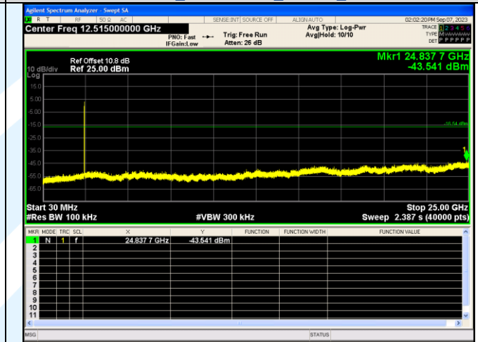
Spurious Emission IEEE 802.11b Channel 11 20MHz Antenna 0
