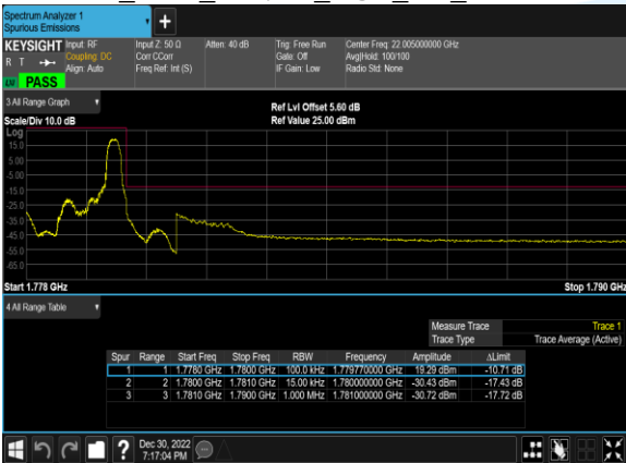
B66_1.4M_64QAM_1@5_CH_132665
