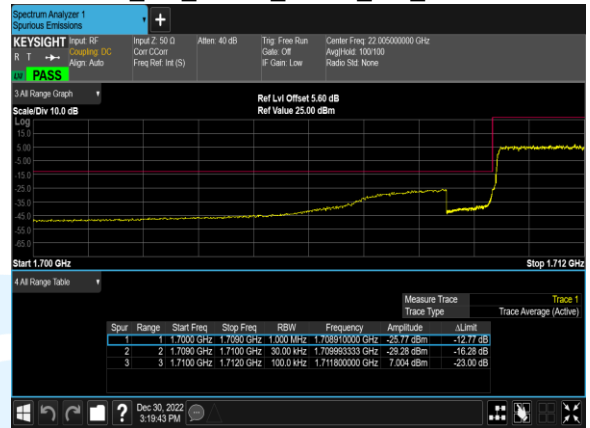
B66_3M_16QAM_15@0_CH_131987
