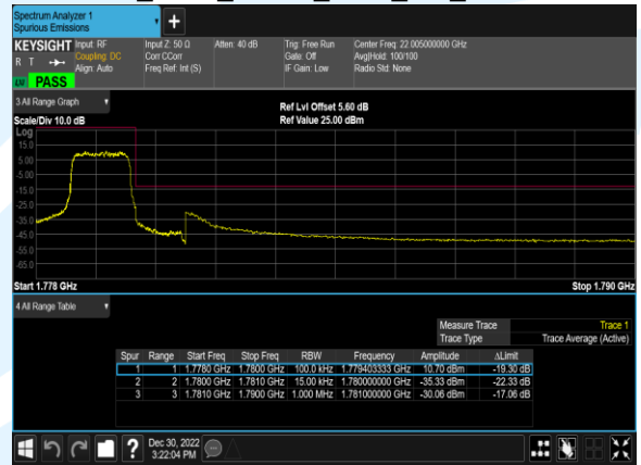
B66_1.4M_16QAM_6@0_CH_132665
