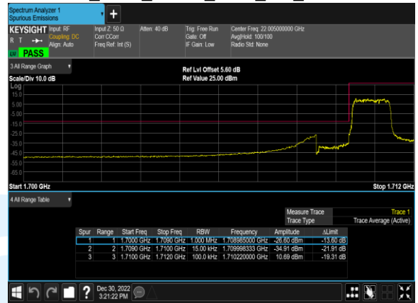
B66_1.4M_16QAM_6@0_CH_131979
