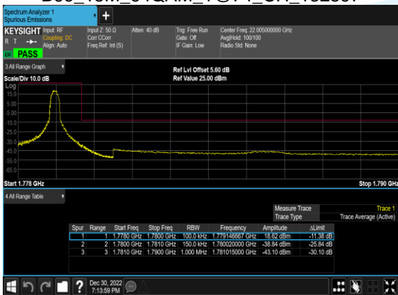
B66_15M_64QAM_1@74_CH_132597
