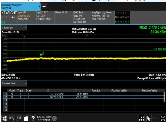
B66_20M_64QAM_1@0_CH_132072
