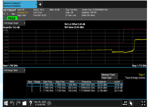
B66_20M_16QAM_100@0_CH_132072
