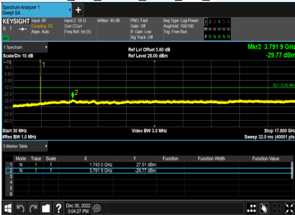
B66_5M_QPSK_1@0_CH_132647
