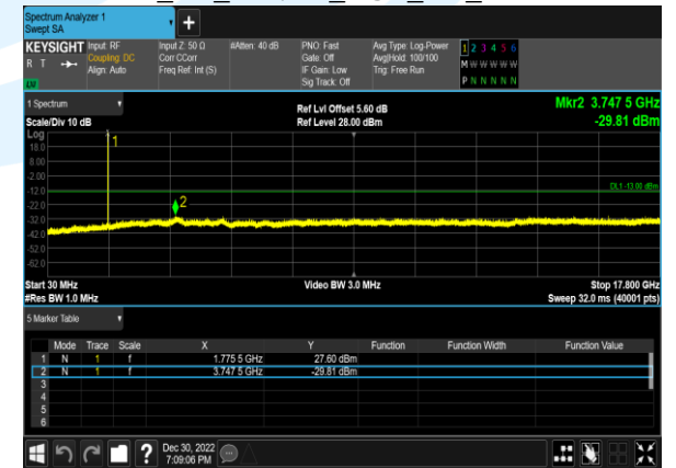
B66_5M_64QAM_1@0_CH_132647
