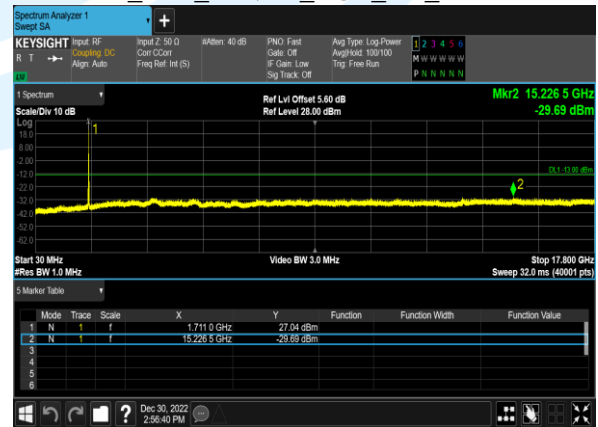
B66_15M_16QAM_1@0_CH_132047
