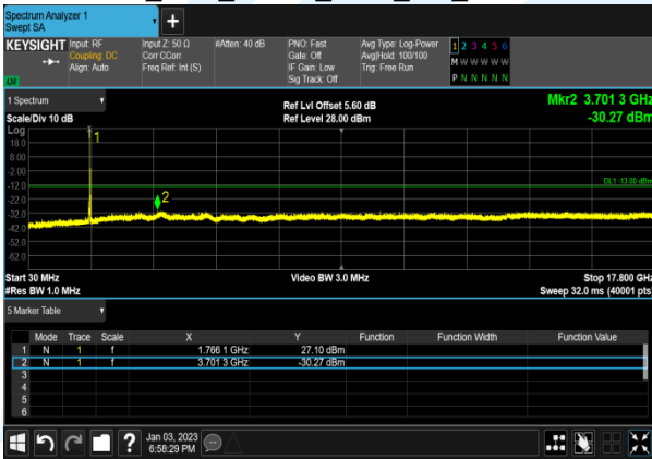
B66_10M_QPSK_1@0_CH_132022
