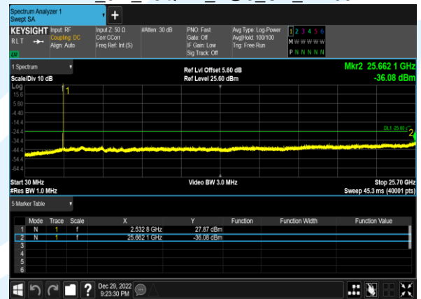
B7_5M_16QAM_1@0_CH_21425
