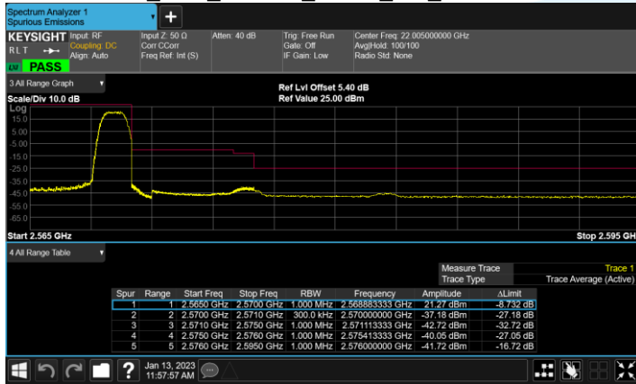
B7_15M_64QAM_1@74_CH_21375
