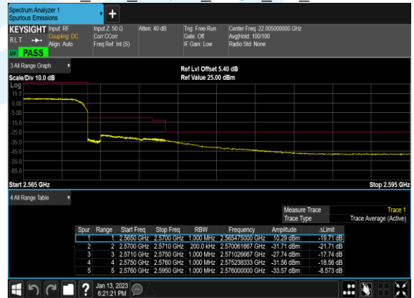
B7_10M_16QAM_50@0_CH_21400
