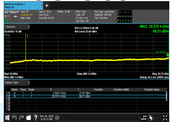
B7_15M_16QAM_1@0_CH_21375
