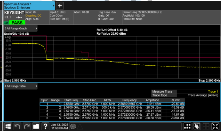
B7_15M_64QAM_75@0_CH_21375
