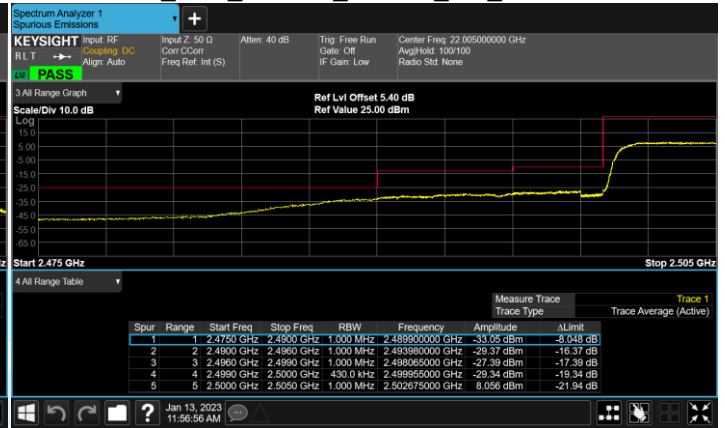
B7_20M_64QAM_100@0_CH_21350
