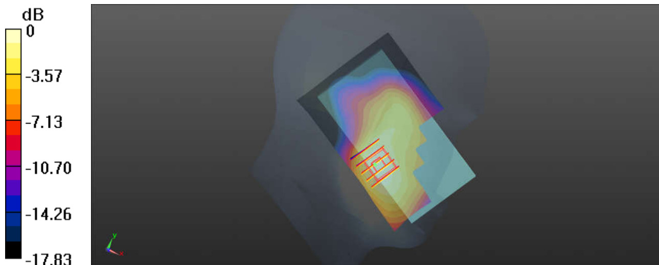
0 dB = 0.577 W/kg
