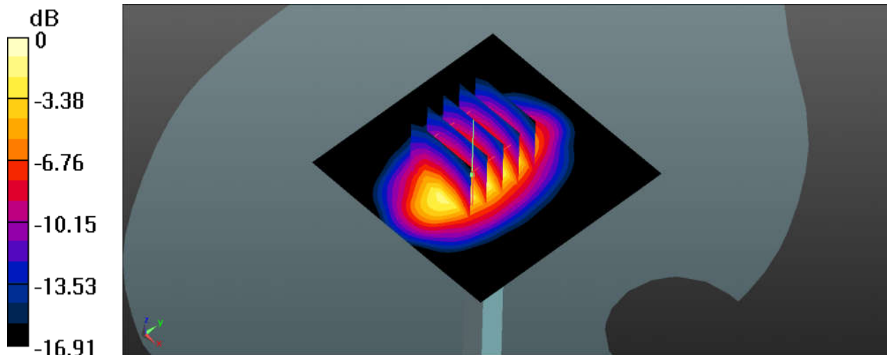
0 dB = 12.4 W/kg
