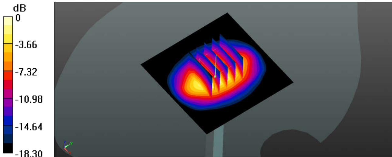
0 dB = 13.7 W/kg
