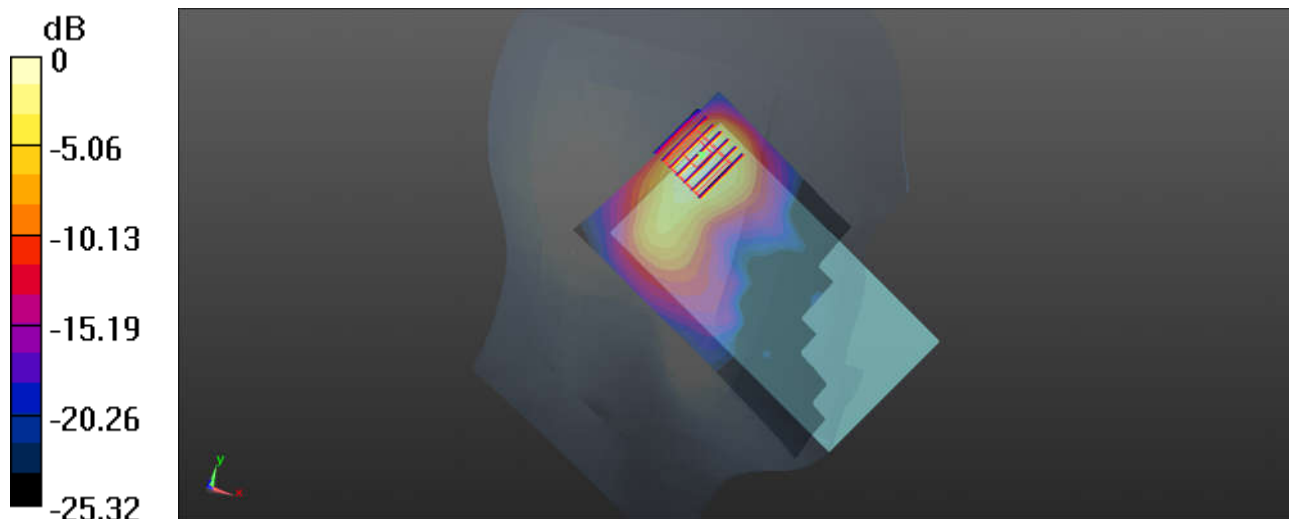
0 dB = 1.05 W/kg
