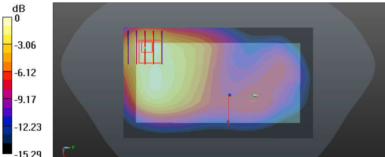
0 dB = 0.773 W/kg
