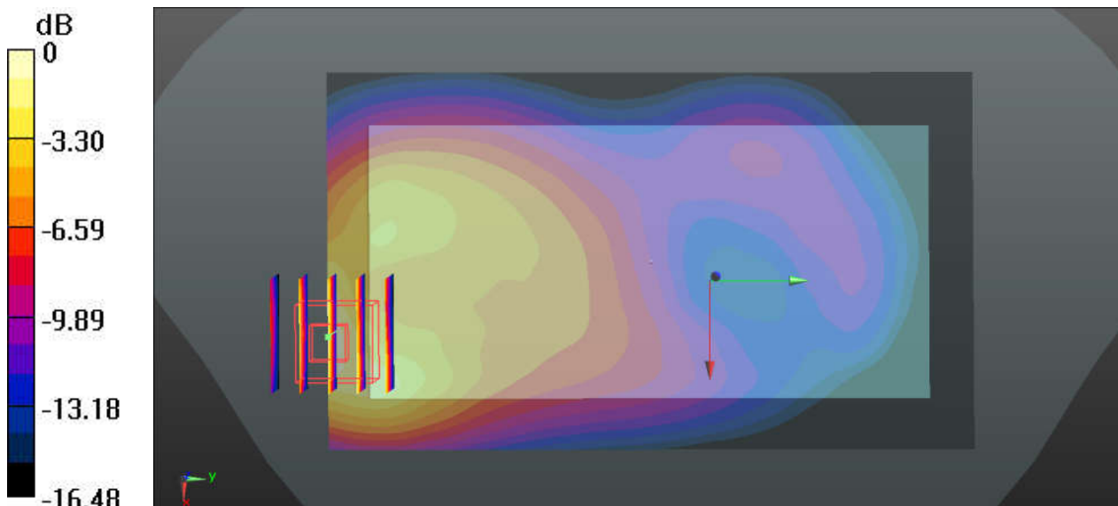
0 dB = 1.03 W/kg
