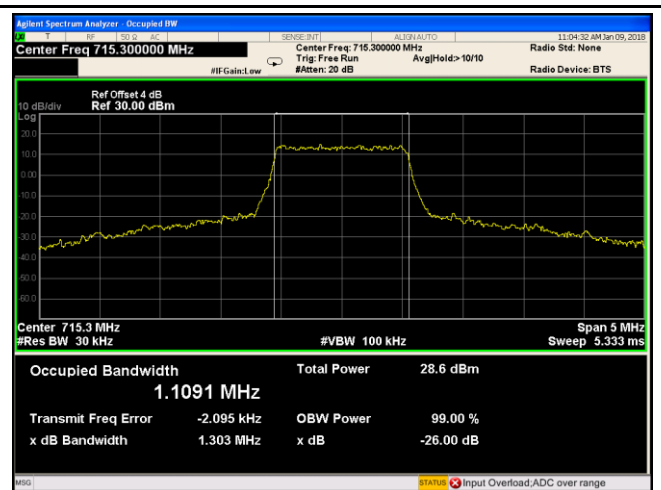
LTE Band XII - High CH 16QAM-1.4
