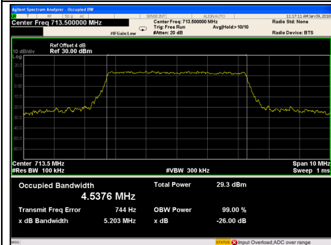
LTE Band XII - High CH QPSK-5
