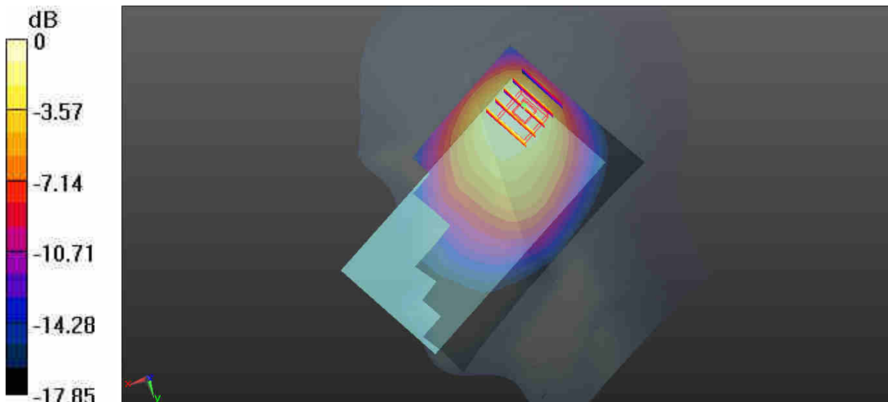
0 dB = 1.41 W/kg
