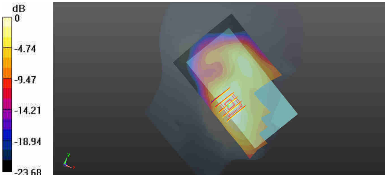
0 dB = 0.358 W/kg
