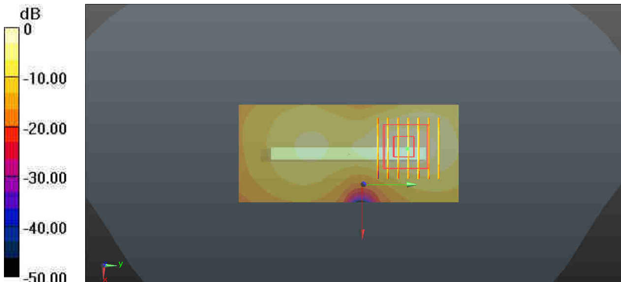
0 dB = 0.818 W/kg
