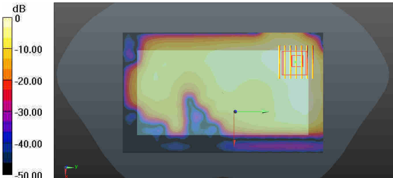
0 dB = 0.140 W/kg
