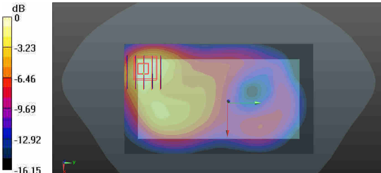
0 dB = 0.867 W/kg
