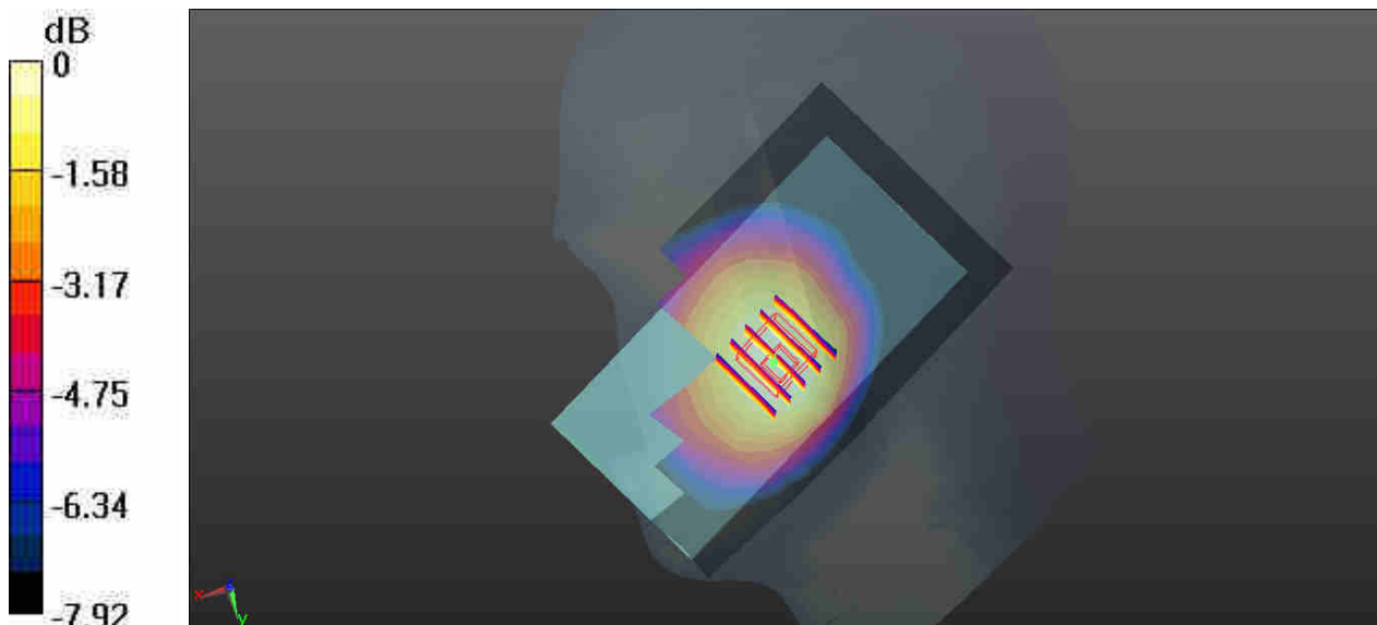
0 dB = 0.168 W/kg
