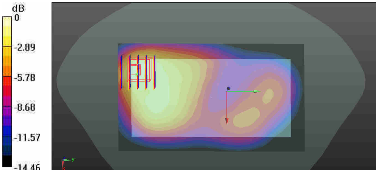
0 dB = 0.778 W/kg
