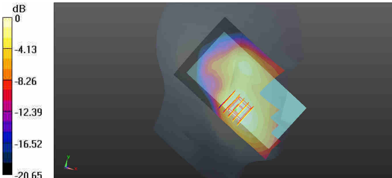
0 dB = 0.310 W/kg
