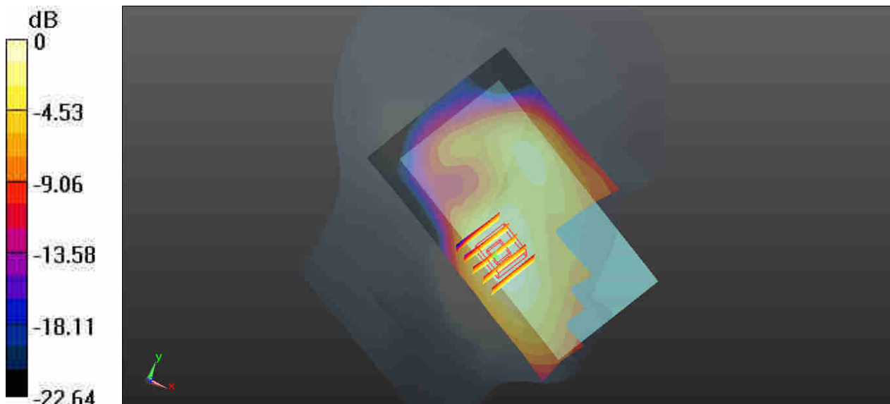
0 dB = 0.325 W/kg
