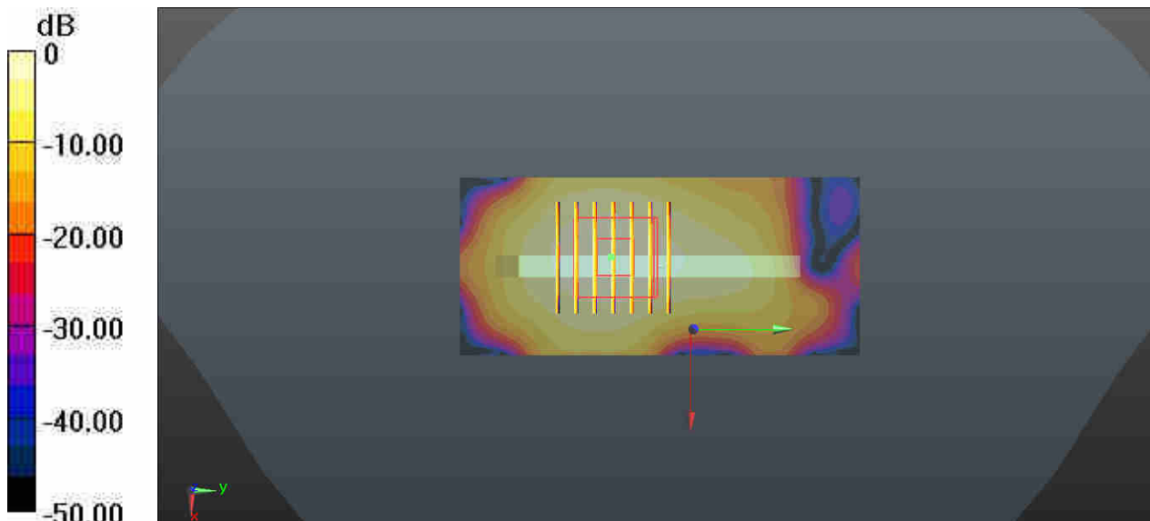
0 dB = 0.166 W/kg
