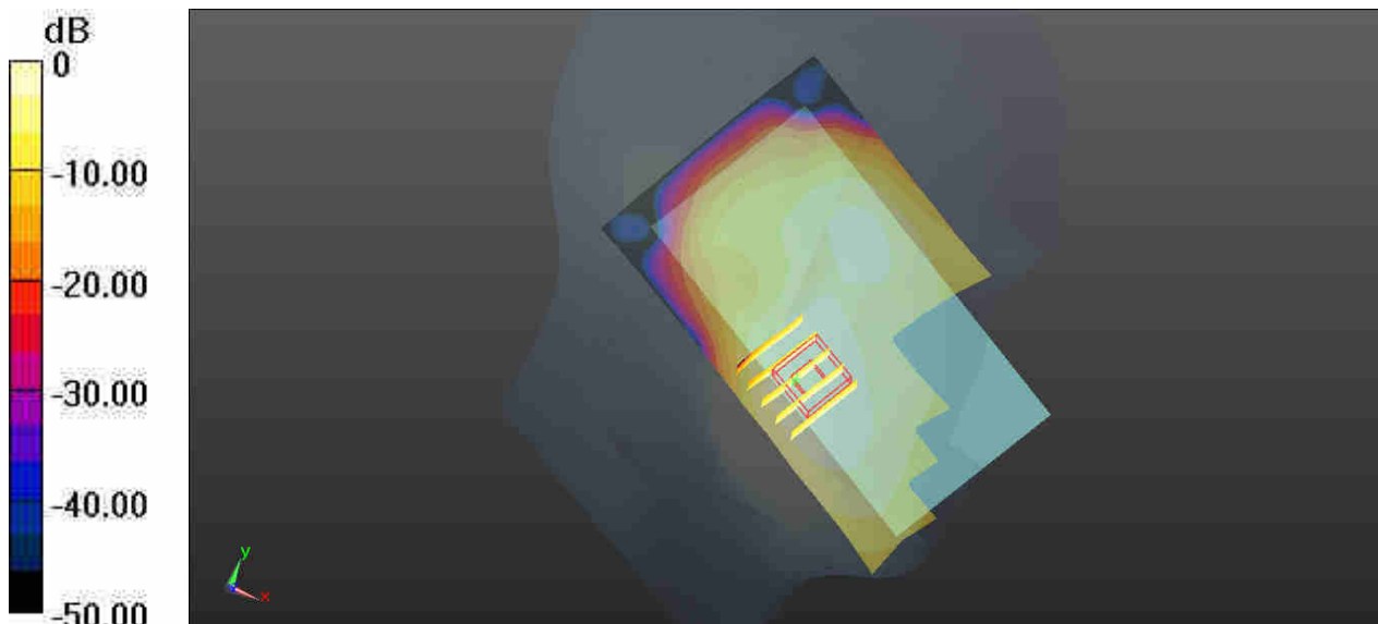
0 dB = 0.263 W/kg
