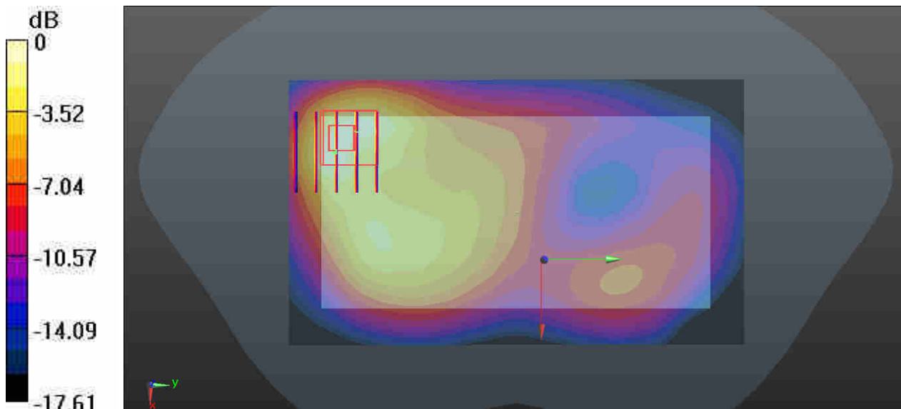
0 dB = 1.11 W/kg
