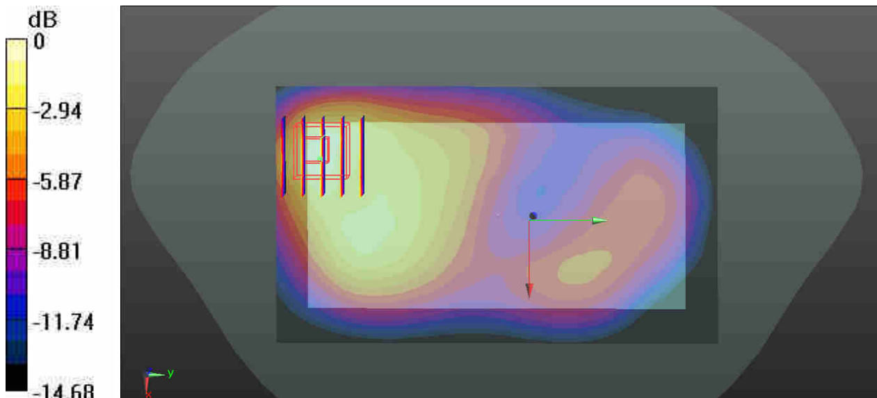
0 dB = 0.667 W/kg
