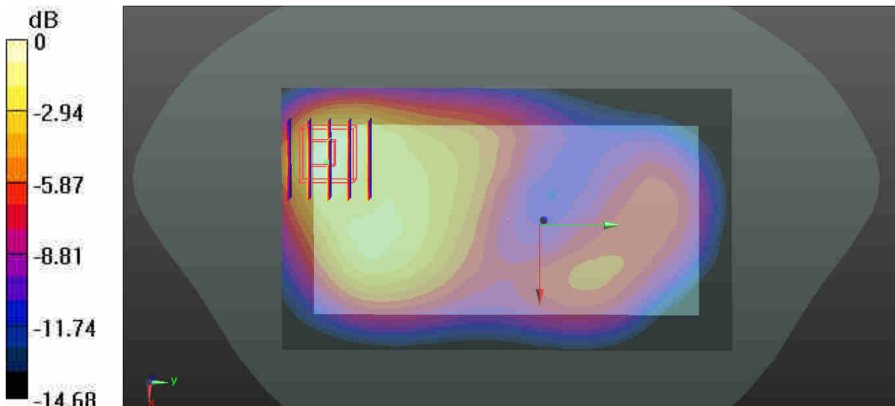
0 dB = 0.667 W/kg
