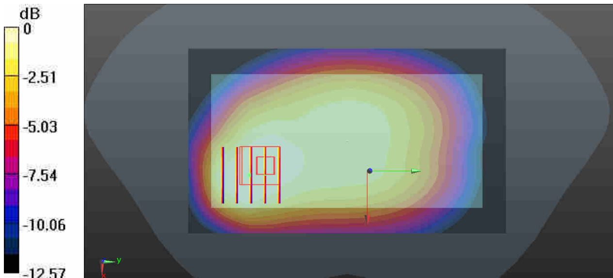
0 dB = 0.282 W/kg
