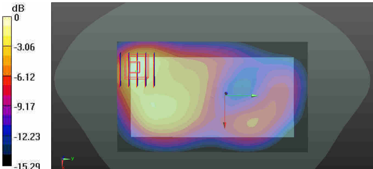
0 dB = 0.860 W/kg
