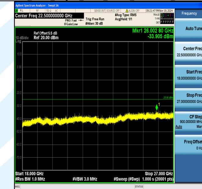
Band7_5MHz_16QAM_21100_1RB#0_18000~27000_18000~27000
