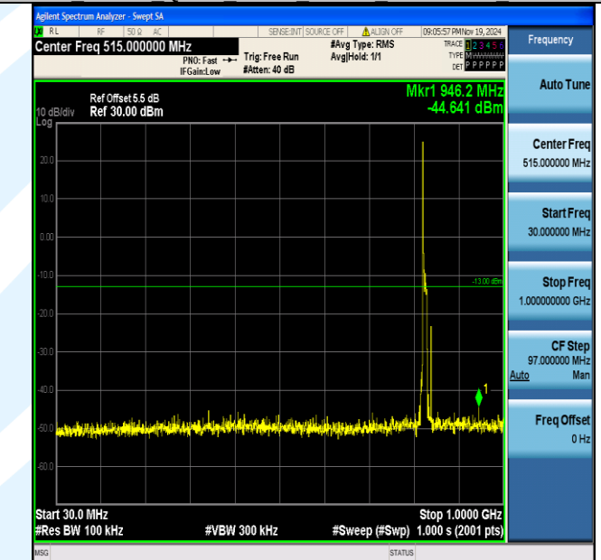
Band5_10MHz_16QAM_20450_1RB#0_30~1000_30~1000
