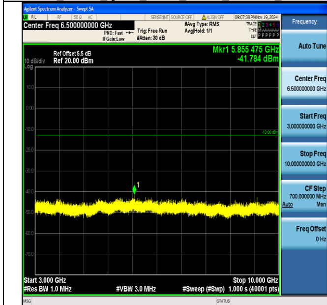
Band5_10MHz_QPSK_20600_1RB#0_3000~10000_3000~10000
