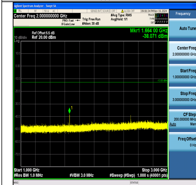
Band5_10MHz_QPSK_20525_1RB#0_1000~3000_1000~3000
