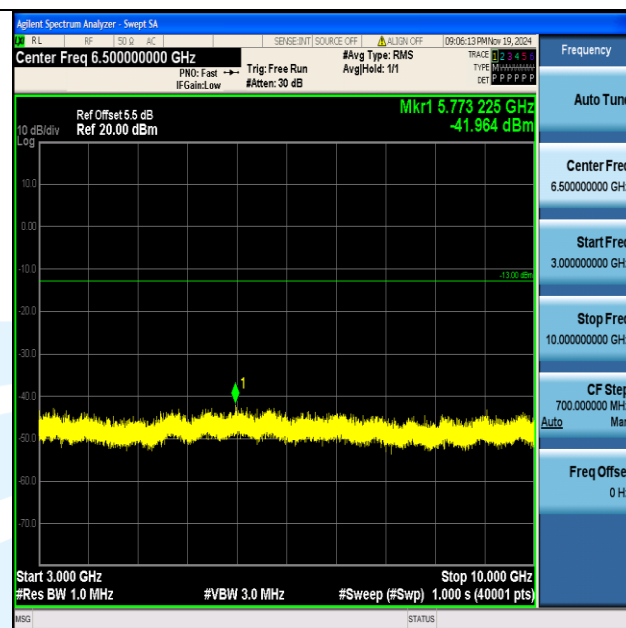
Band5_10MHz_16QAM_20450_1RB#0_3000~10000_3000~10000
