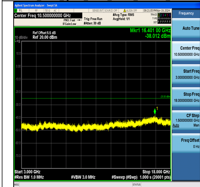
Band7_5MHz_QPSK_21100_1RB#0_3000~18000_3000~18000
