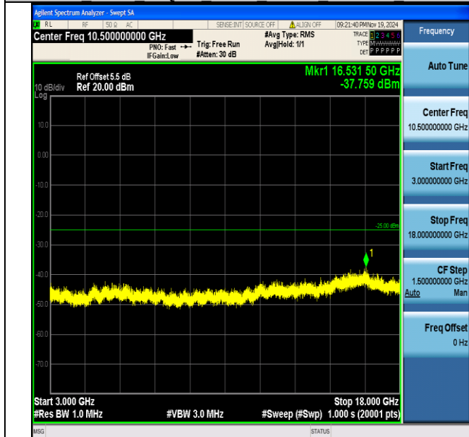
Band7_5MHz_16QAM_21100_1RB#0_3000~18000_3000~18000
