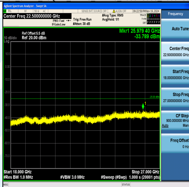
Band7_5MHz_16QAM_21425_1RB#0_18000~27000_18000~27000
