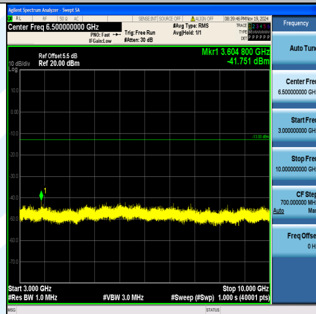
Band5_3MHz_16QAM_20635_1RB#0_3000~10000_3000~10000
