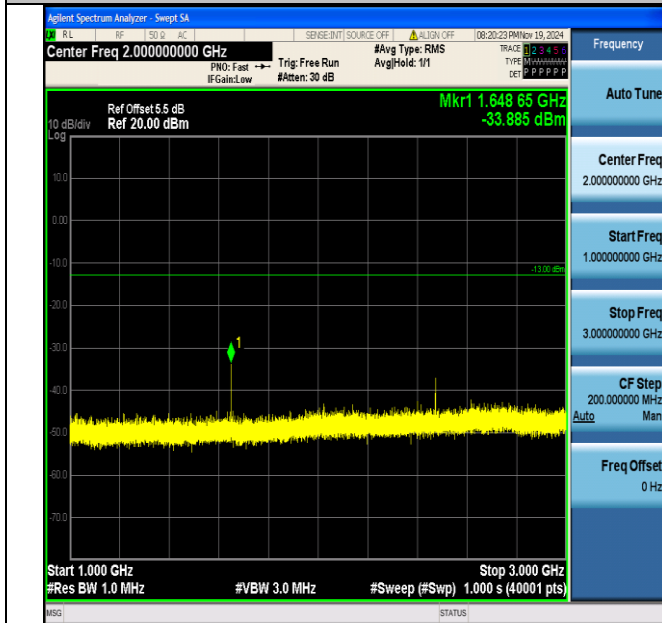
Band5_1.4MHz_16QAM_20407_1RB#0_1000~3000_1000~3000
