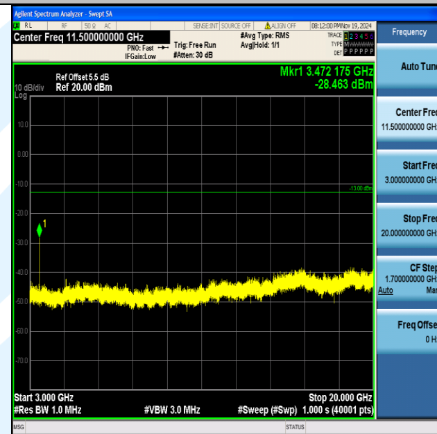
Band4_20MHz_16QAM_20300_1RB#0_3000~20000_3000~20000
