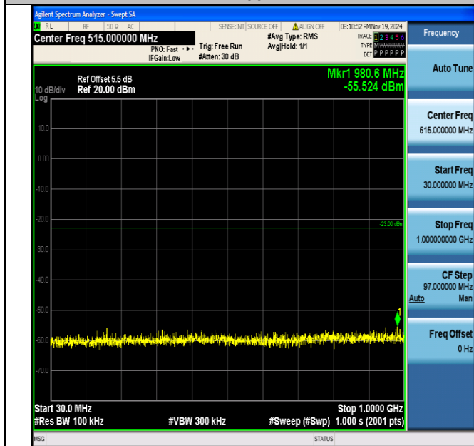
Band4_20MHz_16QAM_20175_1RB#0_30~1000_30~1000
