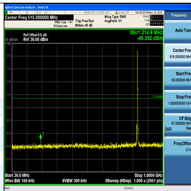
Band5_3MHz_QPSK_20525_1RB#0_30~1000_30~1000
