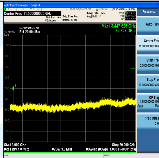
Band4_20MHz_QPSK_20175_1RB#0_3000~20000_3000~20000
