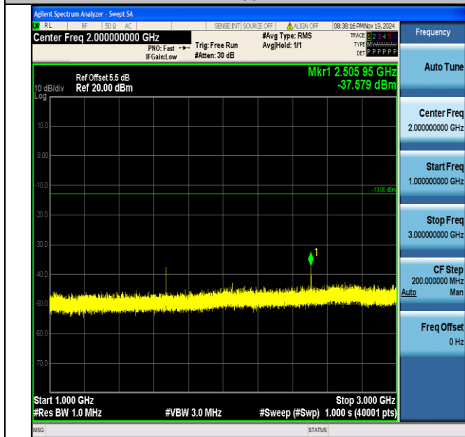
Band5_3MHz_QPSK_20525_1RB#0_1000~3000_1000~3000
