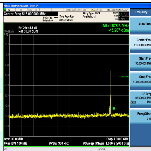
Band5_3MHz_16QAM_20635_1RB#0_30~1000_30~1000
