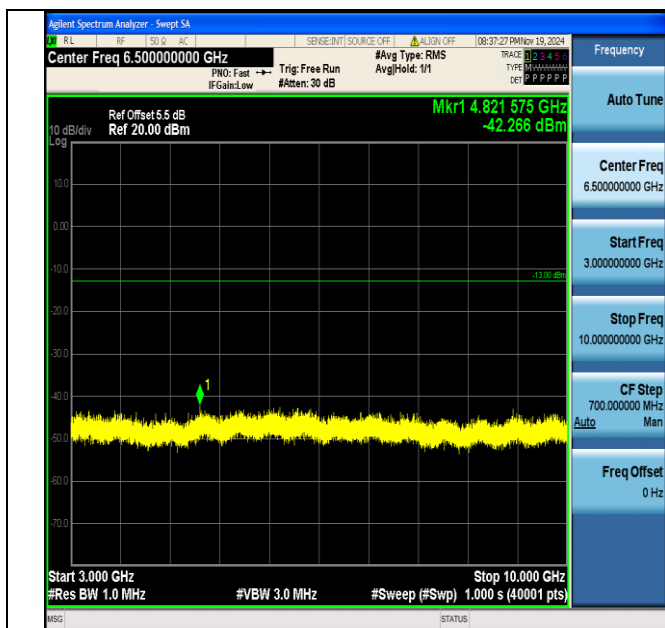
Band5_3MHz_QPSK_20415_1RB#0_3000~10000_3000~10000
