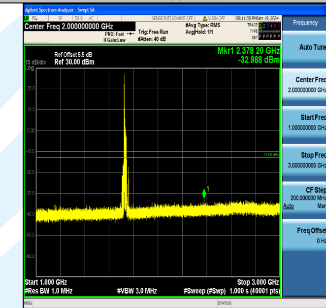
Band4_20MHz_16QAM_20175_1RB#0_1000~3000_1000~3000
