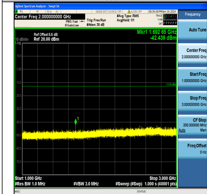
Band5_3MHz_16QAM_20635_1RB#0_1000~3000_1000~3000
