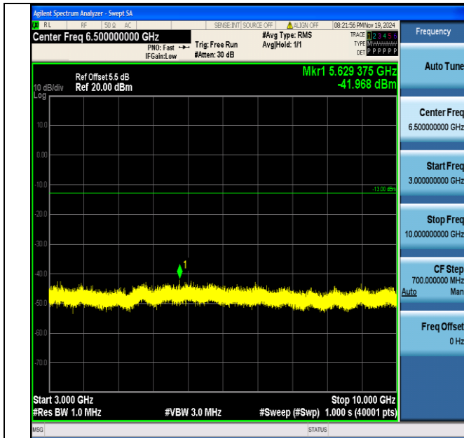
Band5_1.4MHz_QPSK_20643_1RB#0_3000~10000_3000~10000
