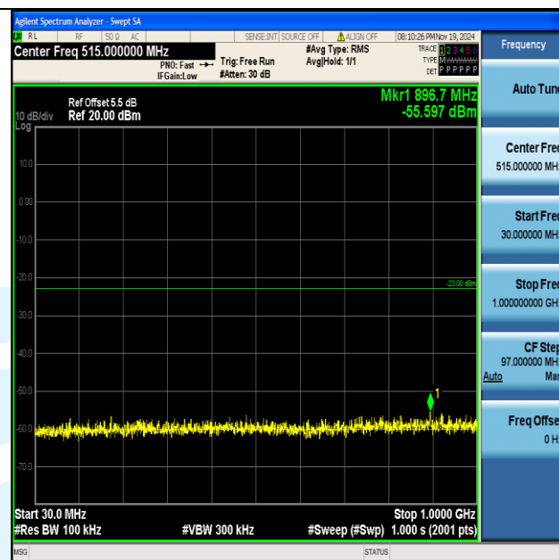
Band4_20MHz_QPSK_20175_1RB#0_30~1000_30~1000
