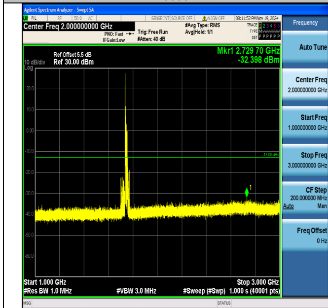
Band4_20MHz_16QAM_20300_1RB#0_1000~3000_1000~3000
