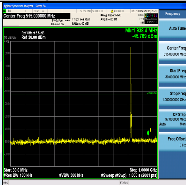
Band5_3MHz_16QAM_20415_1RB#0_30~1000_30~1000
