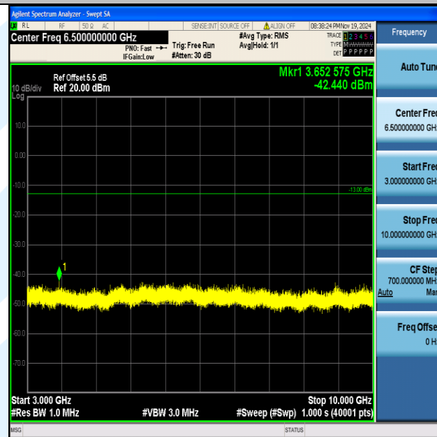
Band5_3MHz_QPSK_20525_1RB#0_3000~10000_3000~10000
