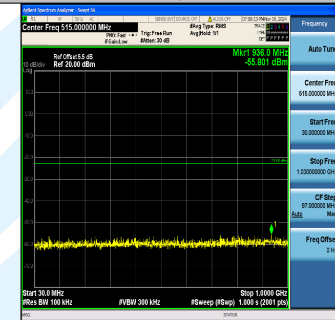
Band4_1.4MHz_16QAM_20393_1RB#0_30~1000_30~1000
