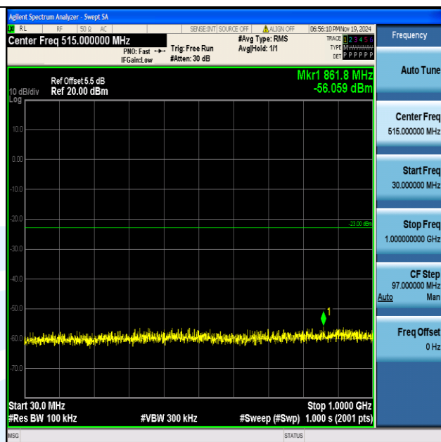
Band2_20MHz_QPSK_18900_1RB#0_30~1000_30~1000
