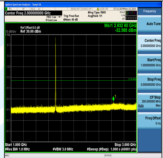
Band4 3MHz QPSK 19965 1RB#0_1000~3000 1000~3000
