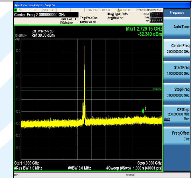
Band2_15MHz_QPSK_19125_1RB#0_1000~3000_1000~3000
