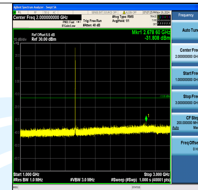
Band4_1.4MHz_16QAM_20175_1RB#0_1000~3000_1000~3000
