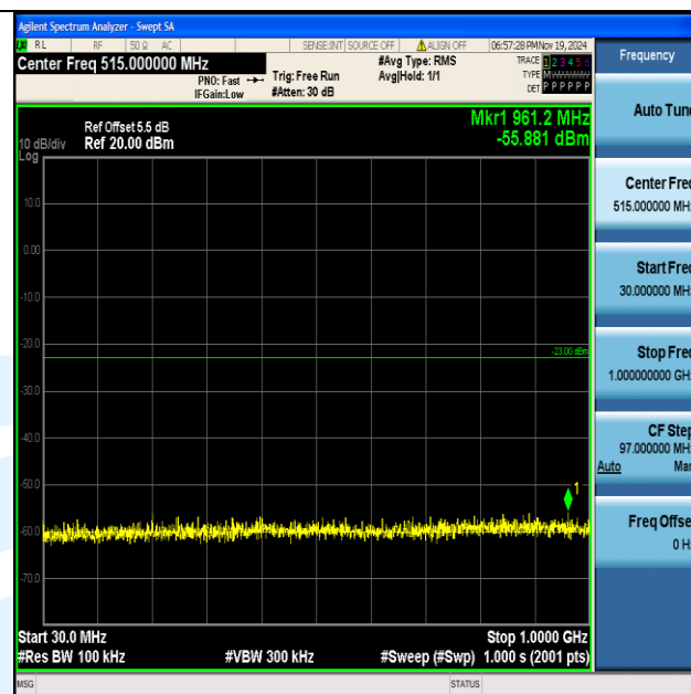
Band2_20MHz_16QAM_19100_1RB#0_30~1000_30~1000
