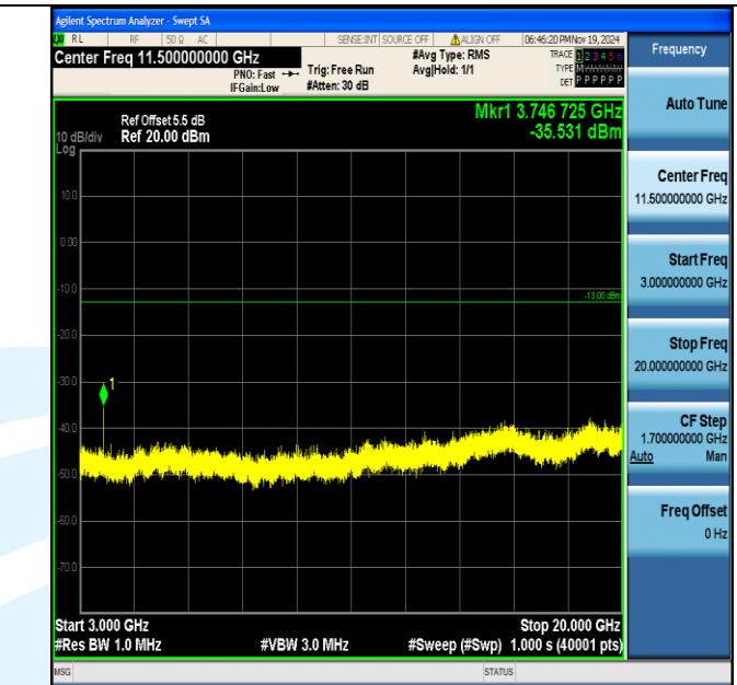
Band2_15MHz_QPSK_18900_1RB#0_3000~20000_3000~20000
