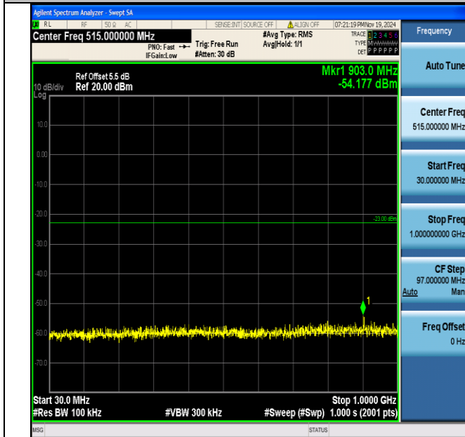
Band4 3MHz QPSK 19965 1RB#0_30~1000 30~1000
