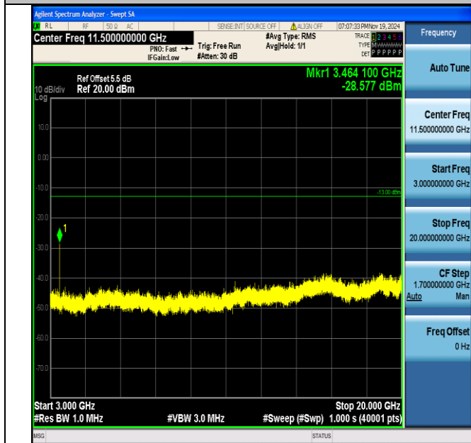
Band4_1.4MHz_16QAM_20175_1RB#0_3000~20000_3000~20000
