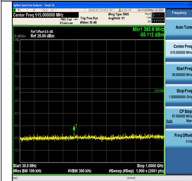
Band2_15MHz_QPSK_19125_1RB#0_30~1000_30~1000
