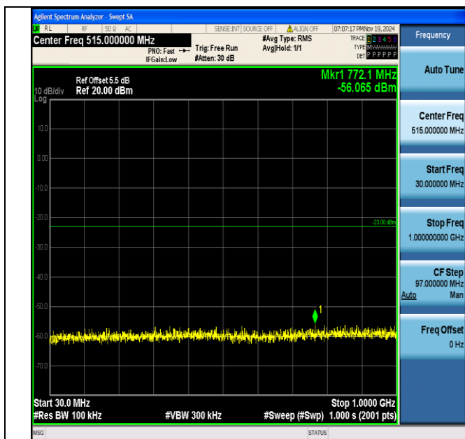
Band4_1.4MHz_16QAM_20175_1RB#0_30~1000_30~1000
