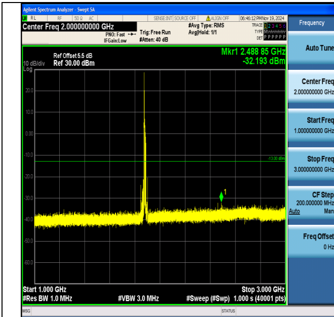
Band2_15MHz_QPSK_18900_1RB#0_1000~3000_1000~3000
