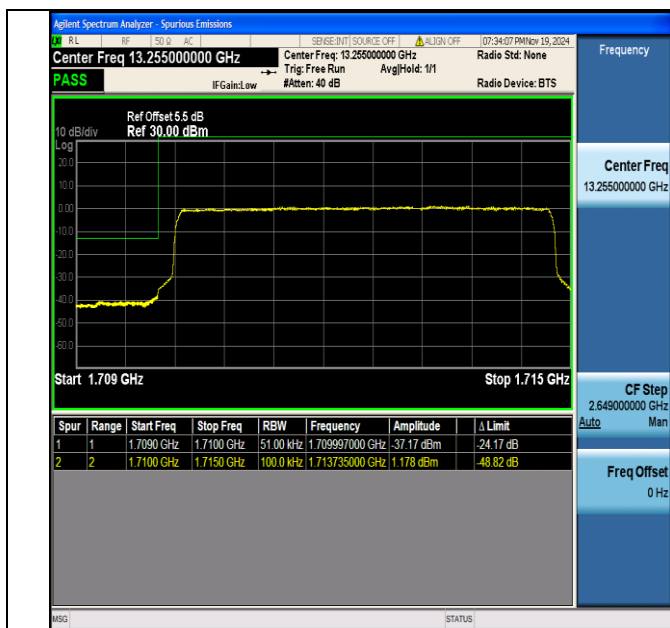
Band4 5MHz 16QAM 19975 25RB#0
