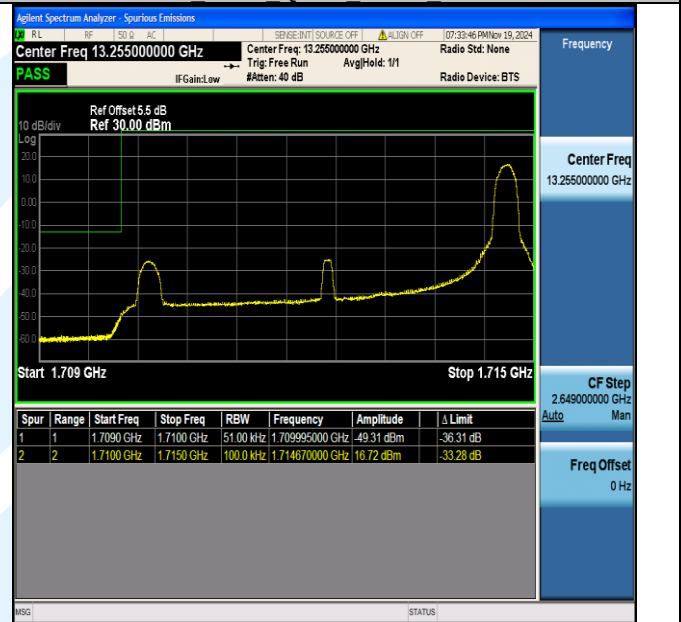
Band4 5MHz 16QAM 19975 1RB#24
