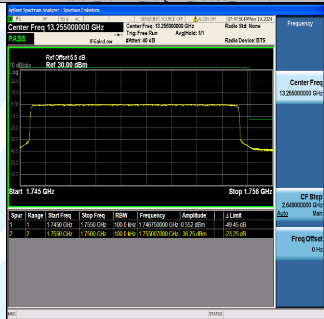
Band4 10MHz 16QAM 20350 50RB#0
