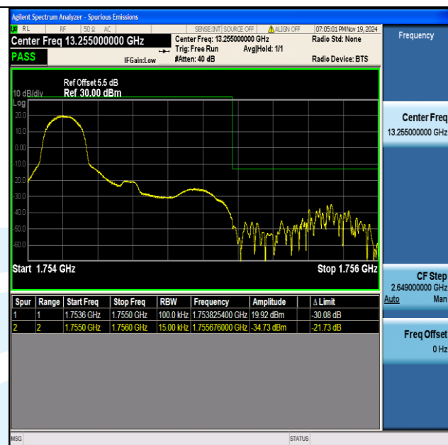
Band4 1.4MHz 16QAM 20393 1RB#0
