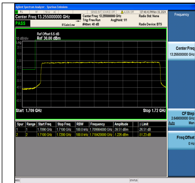
Band4 10MHz 16QAM 20000 50RB#0
