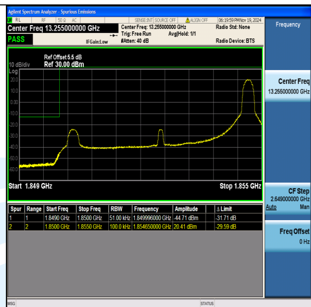
Band2_5MHz_QPSK_18625_1RB#24
