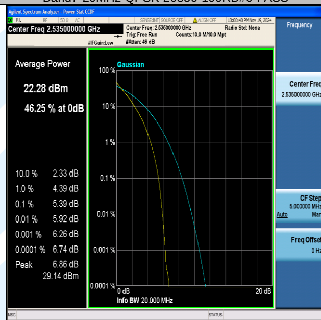
Band7-20MHz-QPSK-21100-100RB#0-PASS
