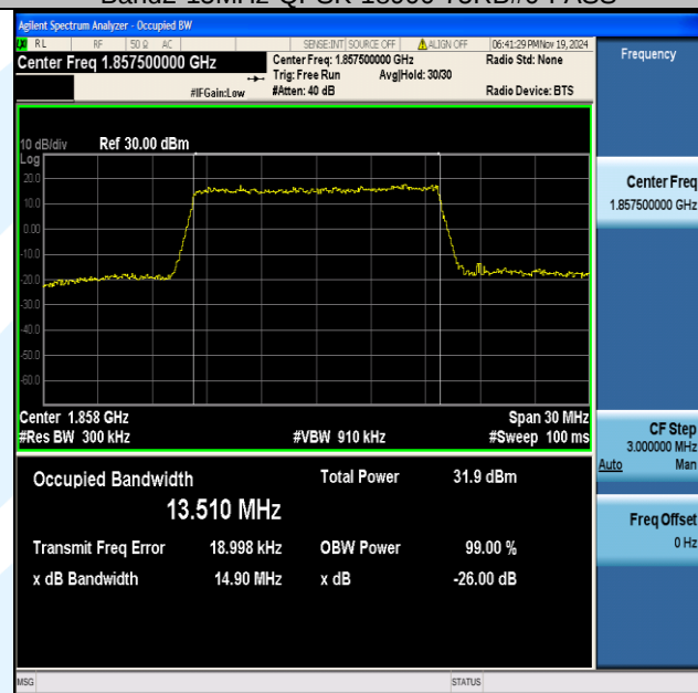
Band2-15MHz-16QAM-18675-75RB#0-PASS
