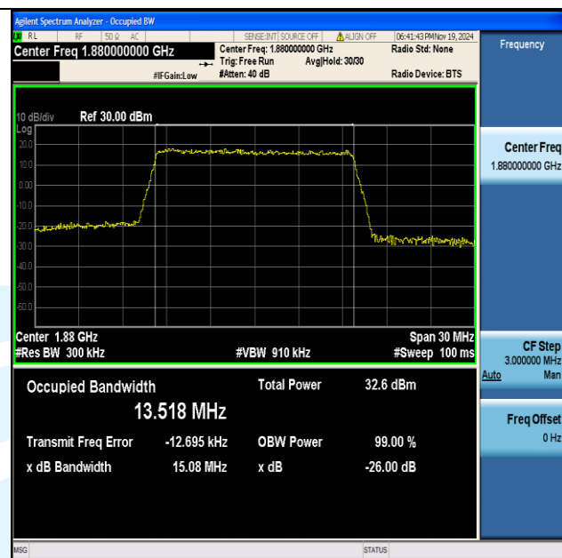
Band2-15MHz-QPSK-18900-75RB#0-PASS
