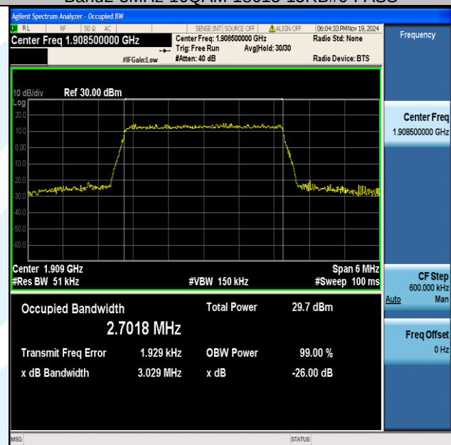
Band2-3MHz-16QAM-19185-15RB#0-PASS
