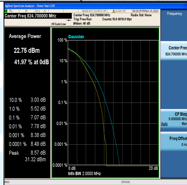
Band5-1.4MHz-16QAM-20407-6RB#0-PASS
