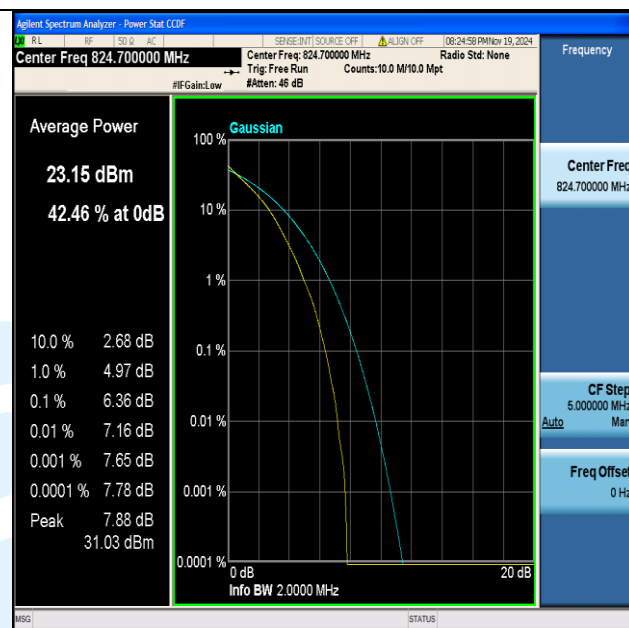
Band5-1.4MHz-QPSK-20407-6RB#0-PASS
