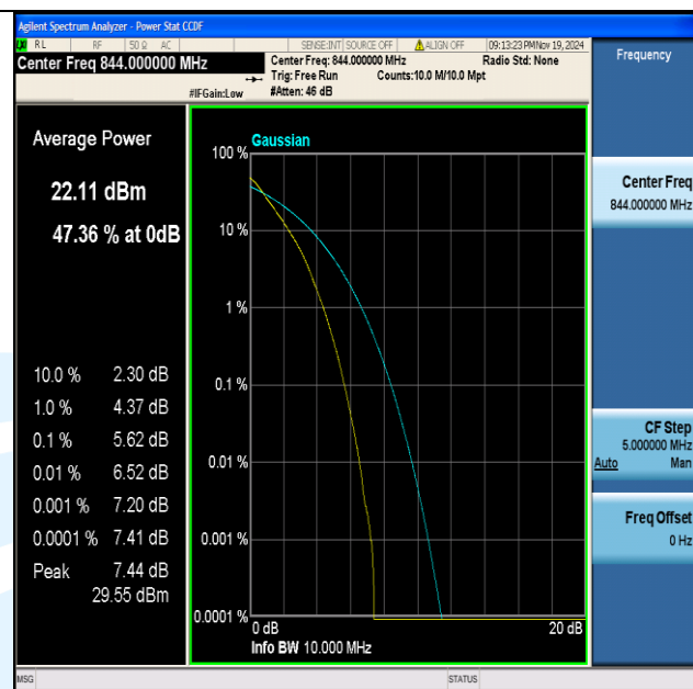
Band5-10MHz-QPSK-20600-50RB#0-PASS
