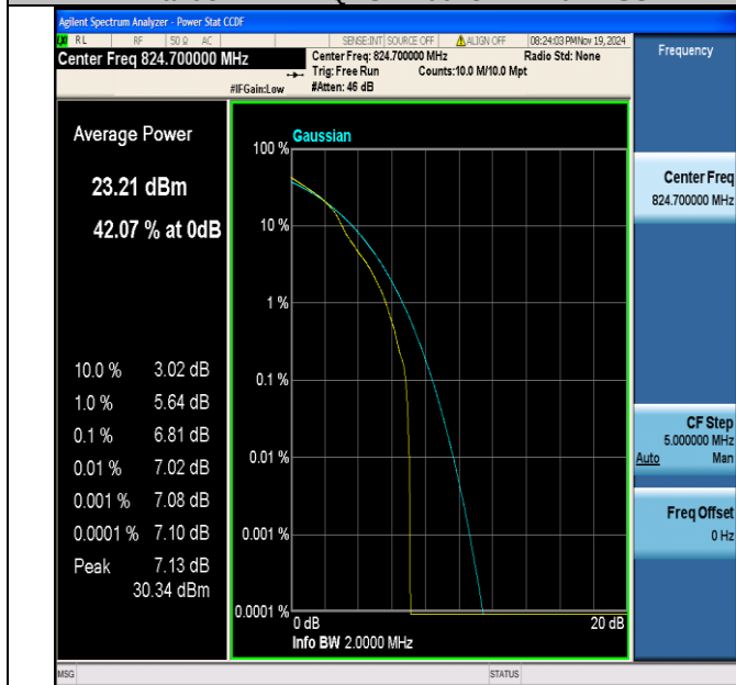
Band5-1.4MHz-16QAM-20407-1RB#0-PASS
