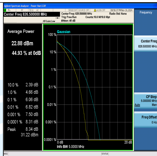
Band5-5MHz-QPSK-20425-25RB#0-PASS
