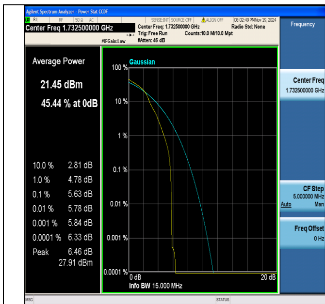
Band4-15MHz-16QAM-20175-1RB#0-PASS
