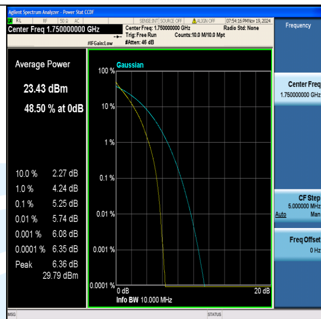
Band4-10MHz-QPSK-20350-50RB#0-PASS
