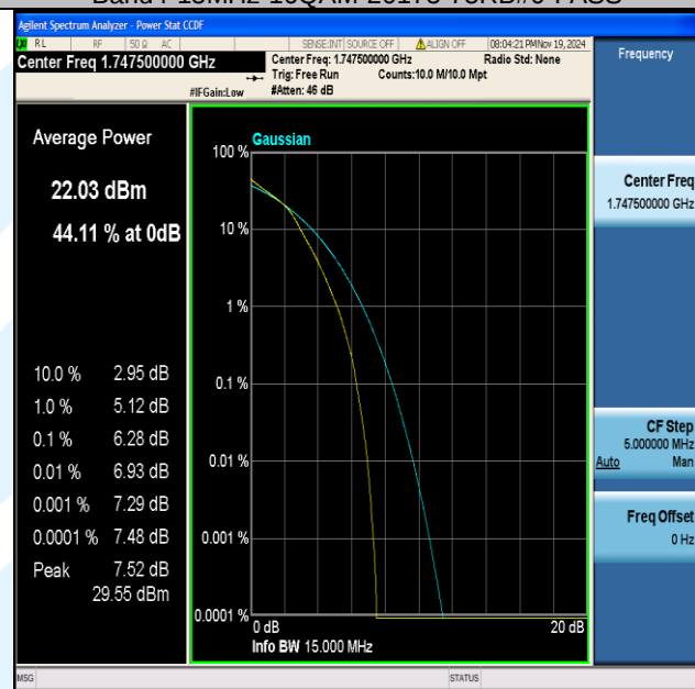
Band4-15MHz-16QAM-20325-75RB#0-PASS
