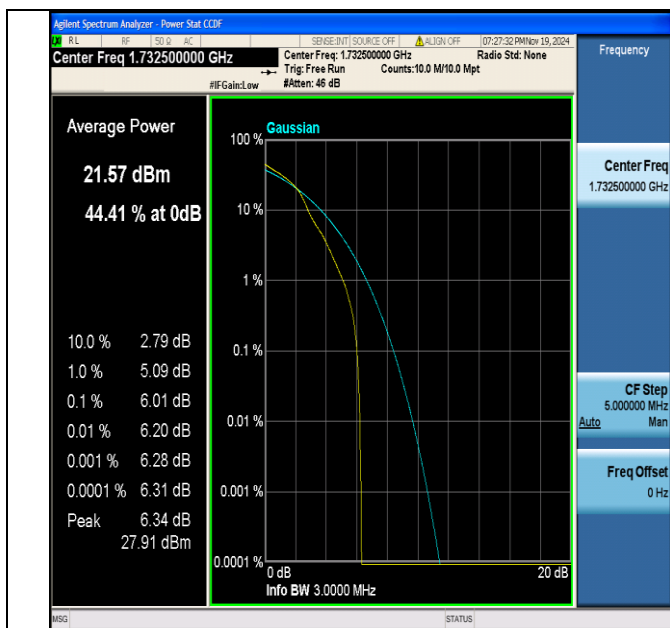
Band4-3MHz-16QAM-20175-1RB#0-PASS
