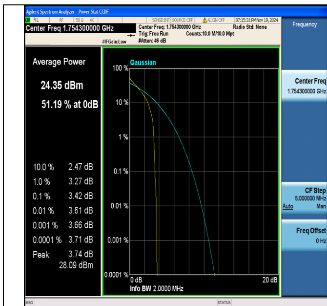
Band4-1.4MHz-QPSK-20393-1RB#0-PASS
