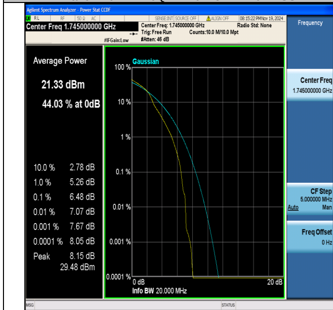
Band4-20MHz-16QAM-20300-1RB#0-PASS
