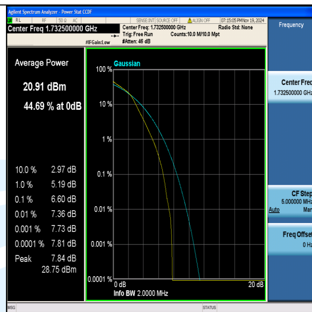
Band4-1.4MHz-16QAM-20175-6RB#0-PASS
