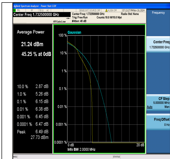
Band4-1.4MHz-16QAM-20175-1RB#0-PASS
