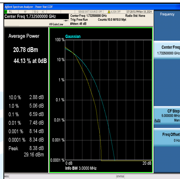
Band4-3MHz-16QAM-20175-15RB#0-PASS
