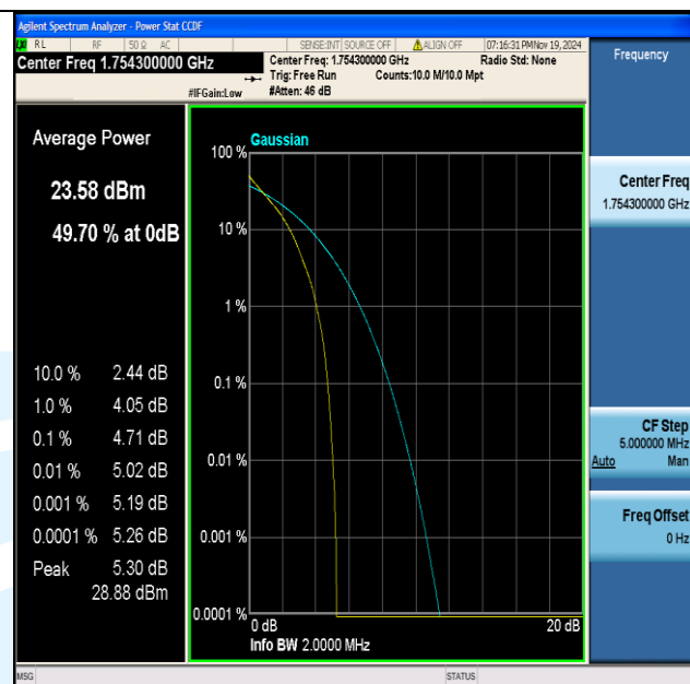
Band4-1.4MHz-QPSK-20393-6RB#0-PASS
