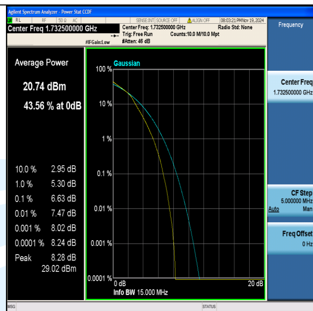
Band4-15MHz-16QAM-20175-75RB#0-PASS
