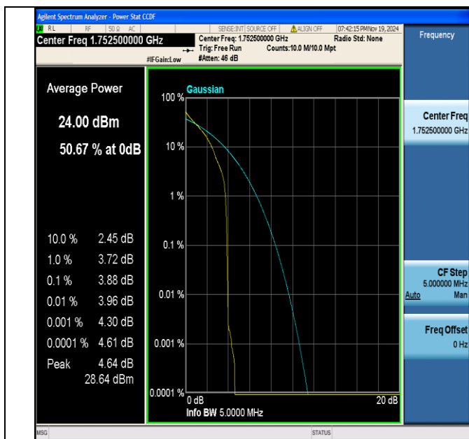
Band4-5MHz-QPSK-20375-1RB#0-PASS
