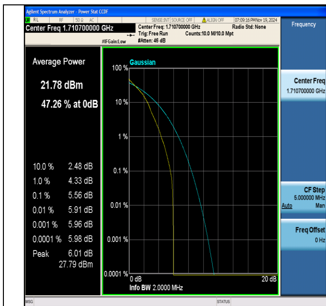
Band4-1.4MHz-QPSK-19957-1RB#0-PASS
