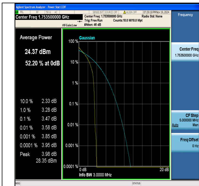
Band4-3MHz-QPSK-20385-1RB#0-PASS
