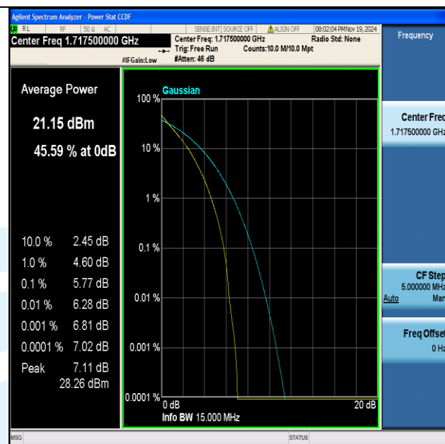
Band4-15MHz-QPSK-20025-75RB#0-PASS
