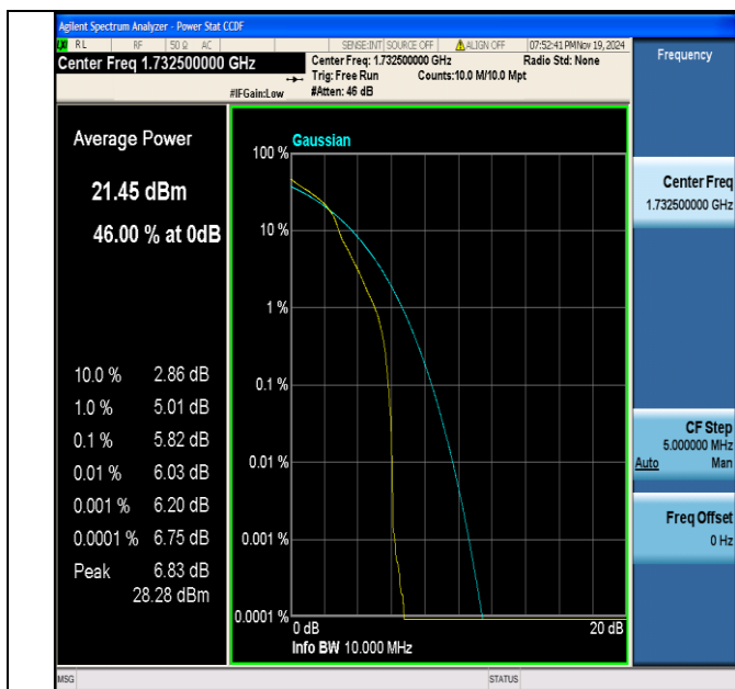
Band4-10MHz-16QAM-20175-1RB#0-PASS
