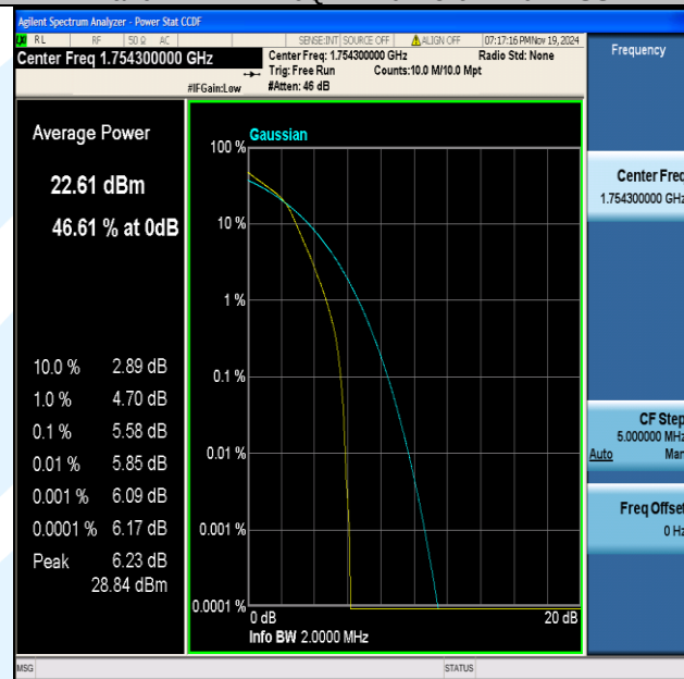
Band4-1.4MHz-16QAM-20393-6RB#0-PASS
