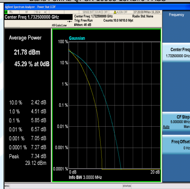
Band4-3MHz-QPSK-20175-15RB#0-PASS
