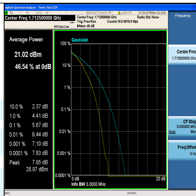
Band4-5MHz-QPSK-19975-25RB#0-PASS
