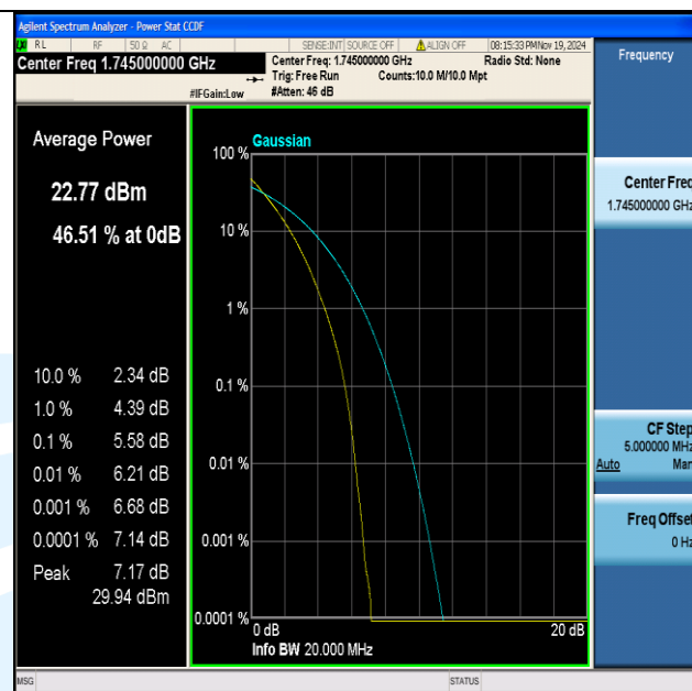
Band4-20MHz-QPSK-20300-100RB#0-PASS
