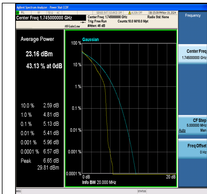
Band4-20MHz-QPSK-20300-1RB#0-PASS
