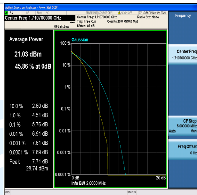
Band4-1.4MHz-QPSK-19957-6RB#0-PASS
