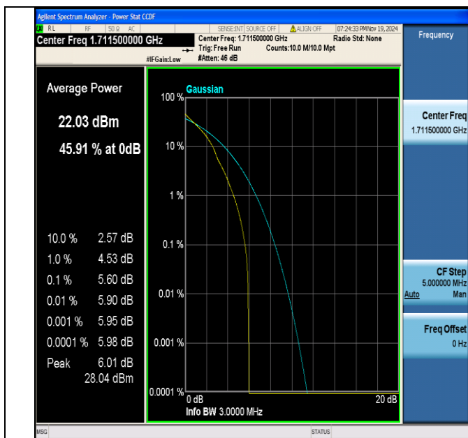
Band4-3MHz-QPSK-19965-1RB#0-PASS
