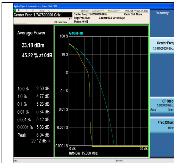
Band4-15MHz-QPSK-20325-1RB#0-PASS
