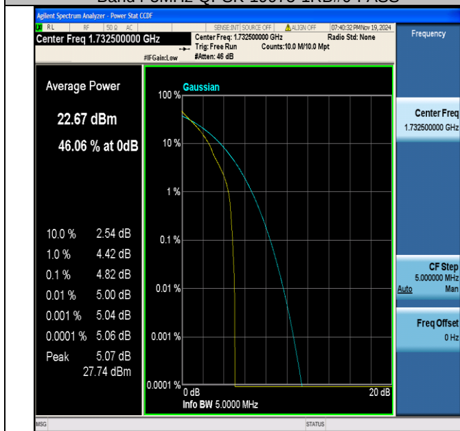
Band4-5MHz-QPSK-20175-1RB#0-PASS
