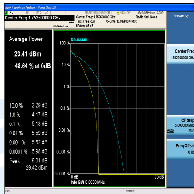
Band4-5MHz-QPSK-20375-25RB#0-PASS
