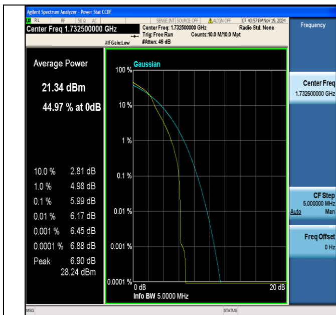
Band4-5MHz-16QAM-20175-1RB#0-PASS
