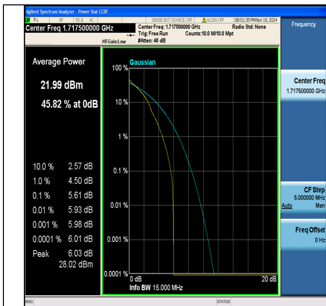
Band4-15MHz-QPSK-20025-1RB#0-PASS
