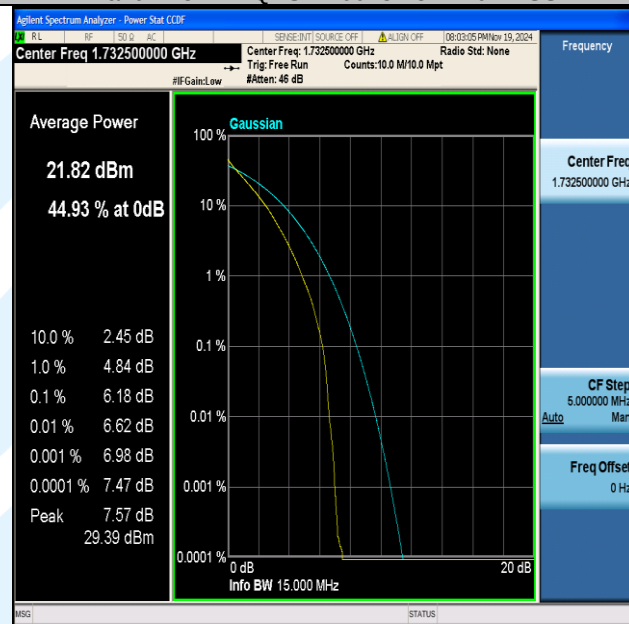
Band4-15MHz-QPSK-20175-75RB#0-PASS
