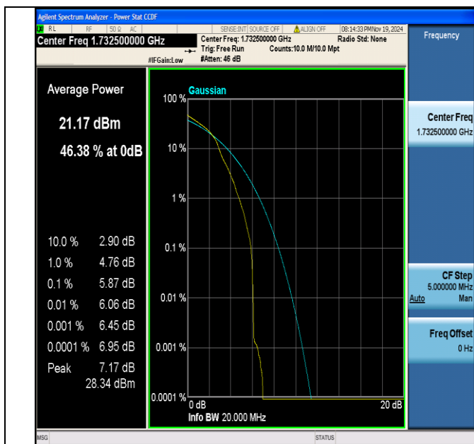
Band4-20MHz-16QAM-20175-1RB#0-PASS
