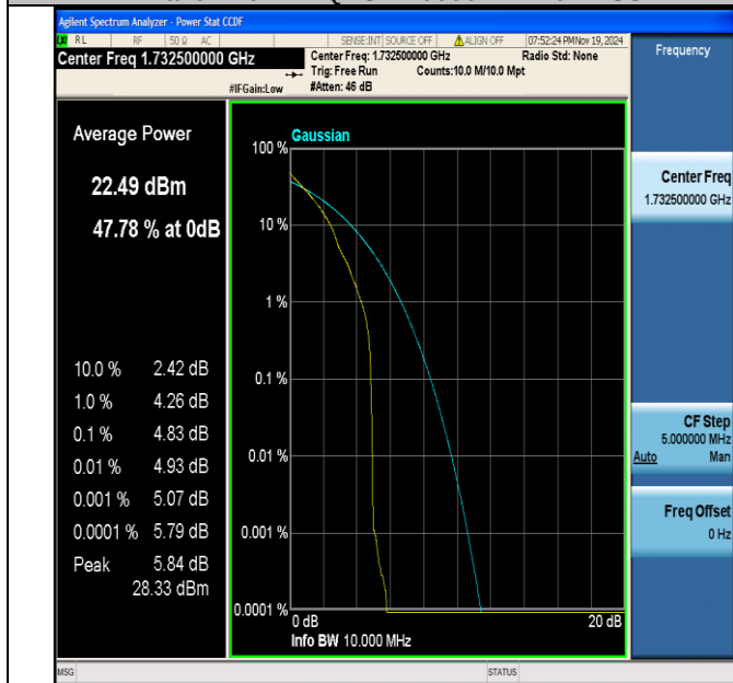
Band4-10MHz-QPSK-20175-1RB#0-PASS
