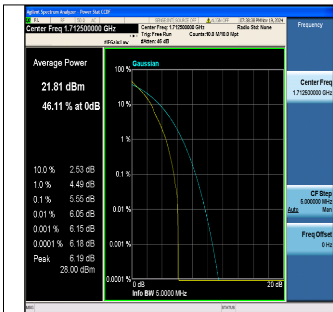
Band4-5MHz-QPSK-19975-1RB#0-PASS
