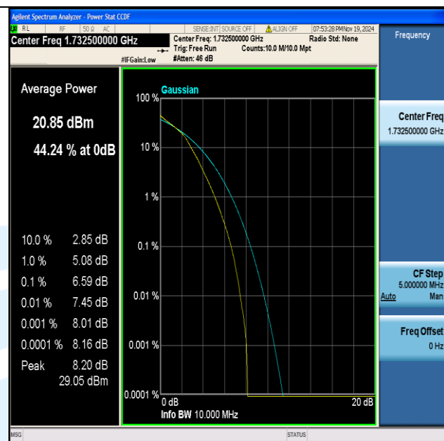
Band4-10MHz-16QAM-20175-50RB#0-PASS
