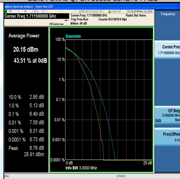
Band4-3MHz-16QAM-19965-15RB#0-PASS
