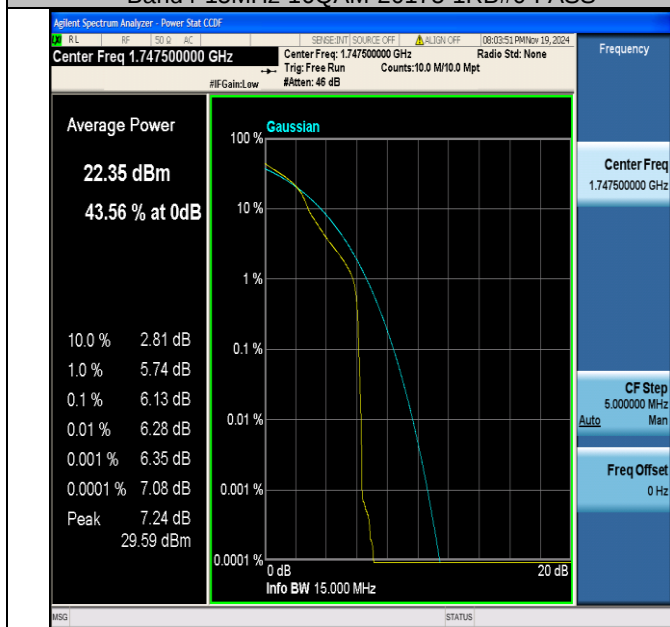
Band4-15MHz-16QAM-20325-1RB#0-PASS
