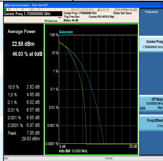
Band4-10MHz-16QAM-20350-50RB#0-PASS
