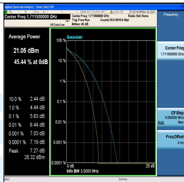
Band4-3MHz-QPSK-19965-15RB#0-PASS
