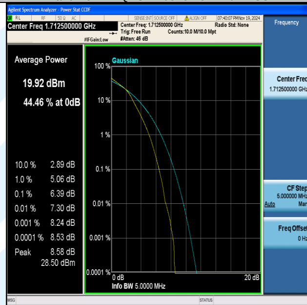
Band4-5MHz-16QAM-19975-25RB#0-PASS
