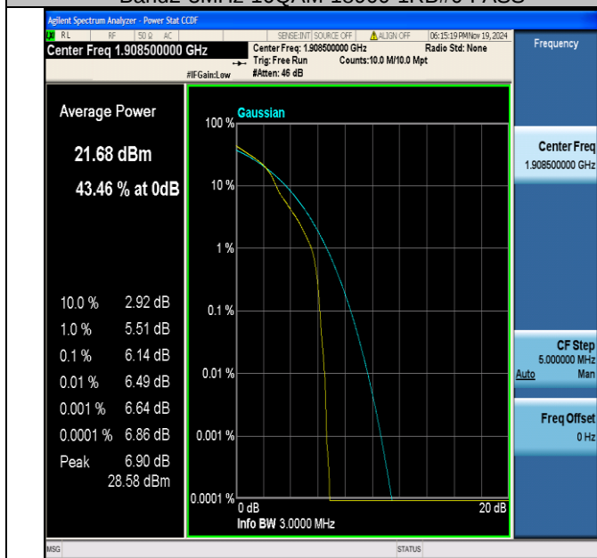
Band2-3MHz-16QAM-19185-1RB#0-PASS
