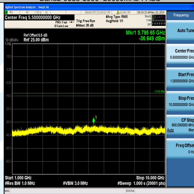
Band5-4132-1000~10000MHz-PASS
