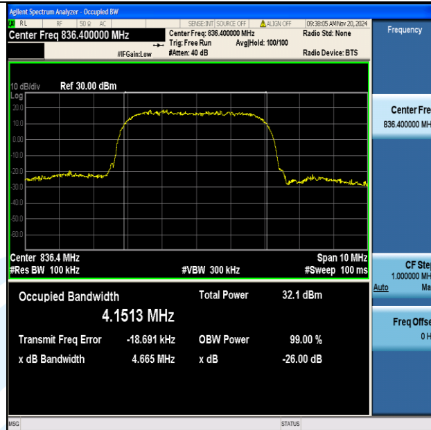
Band5-4182-1-PASS
