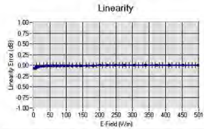
Linearity [ +/- 1.69% (+/- 0.07dB) ]
