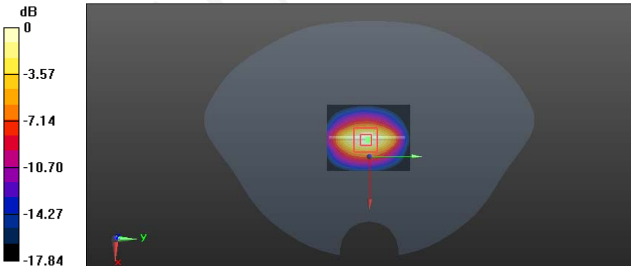
0 dB = 6.12 W/kg = 7.87 dBW/kg
