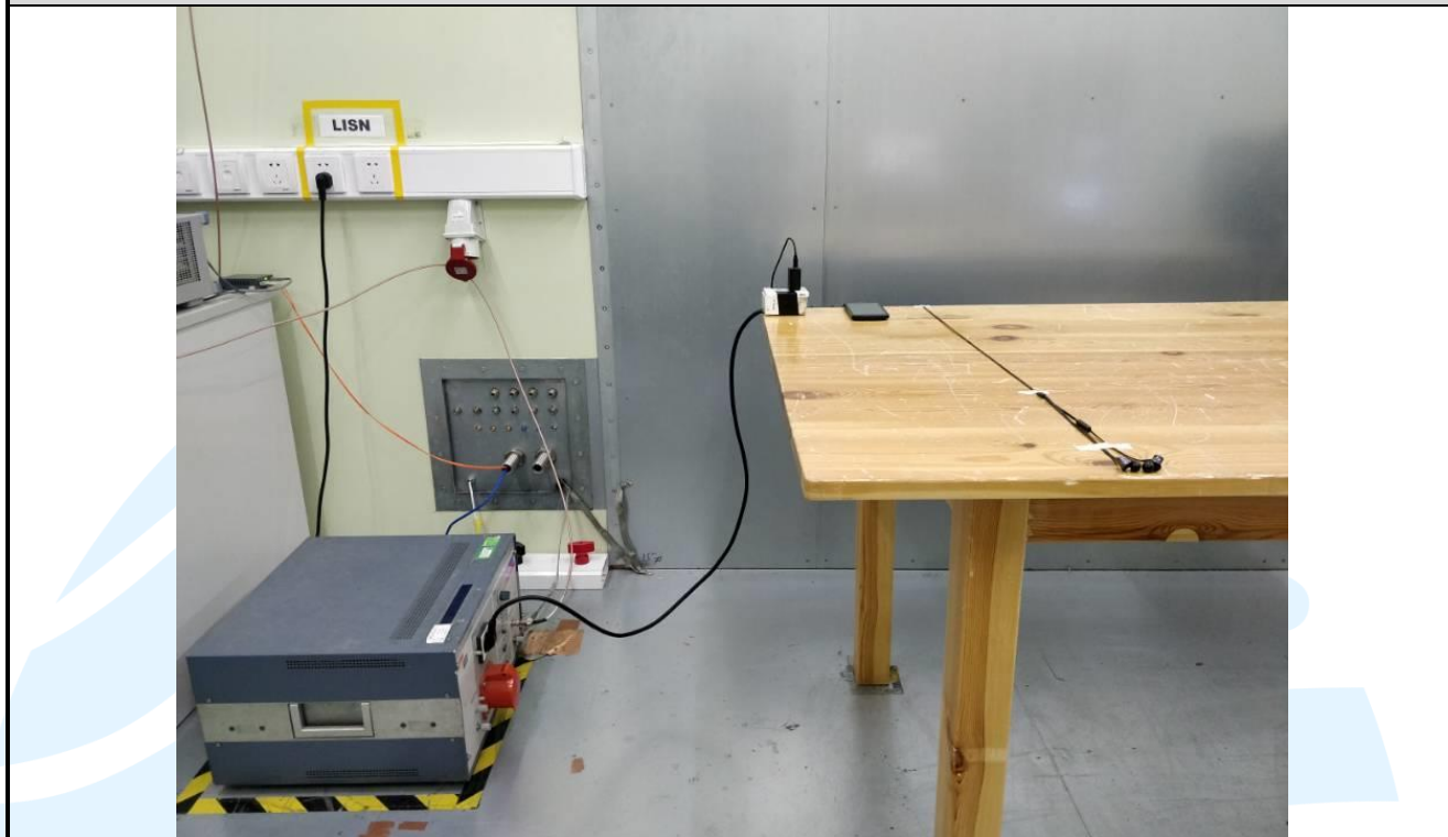
Conducted Emission Test Setup - Mode 4
